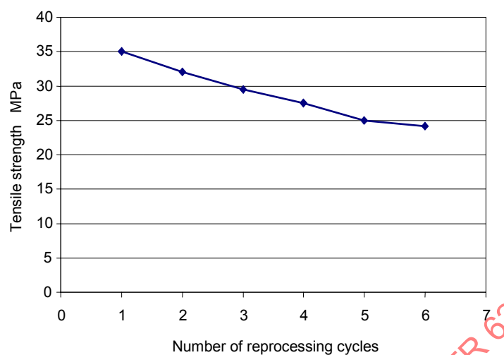
Figure 3 – Tensile strength of reprocessed material
