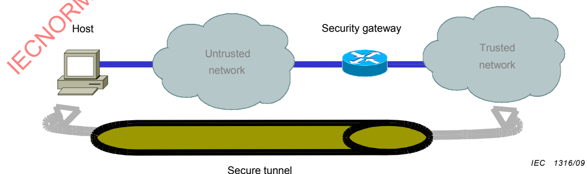
Figure 3 – Host to security gateway VPN
