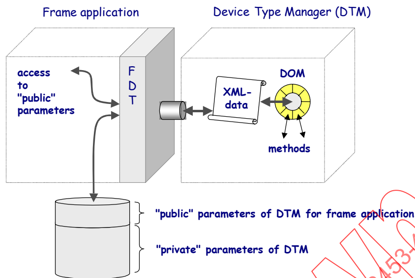
Figure 5 – Data access and storage
