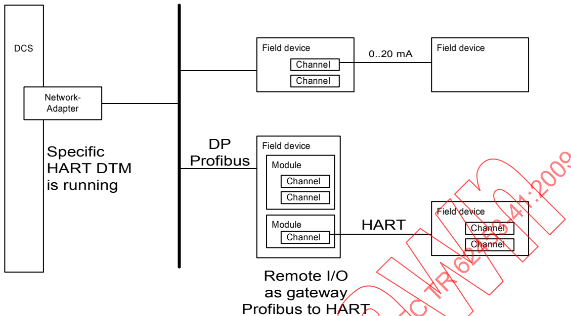
Figure 20 – System-topology
