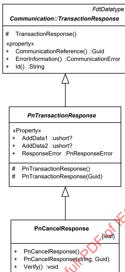
Figure 14 – PnCancelResponse
