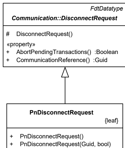
Figure 7 – PnDisconnectRequest
