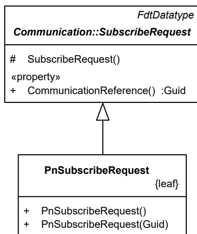
Figure 15 – PnSubscribeRequest
