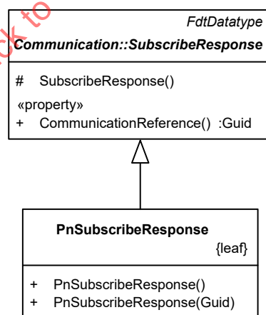
Figure 16 – PnSubscribeResponse
