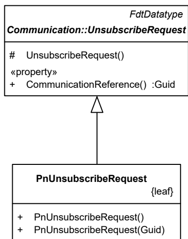
Figure 17 – PnUnsubscribeRequest
