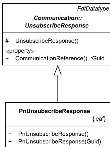
Figure 18 – PnUnsubscribeResponse
