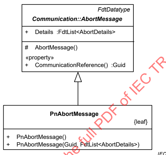
Figure 19 – PnAbortMessage
