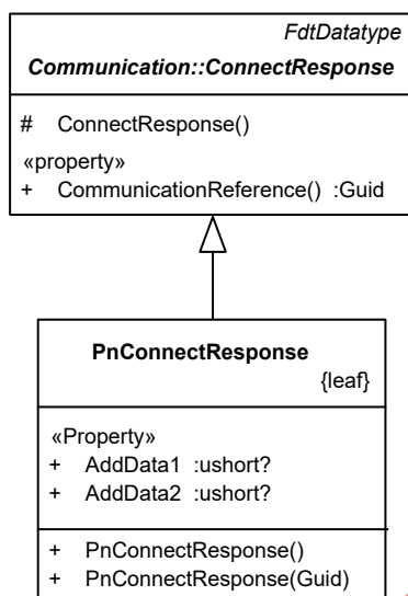
Figure 6 – PnConnectResponse
