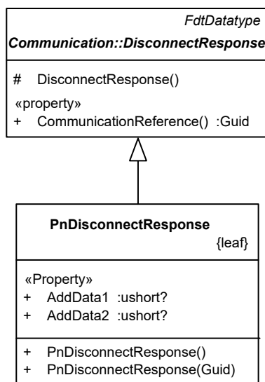
Figure 8 – PnDisconnectResponse
