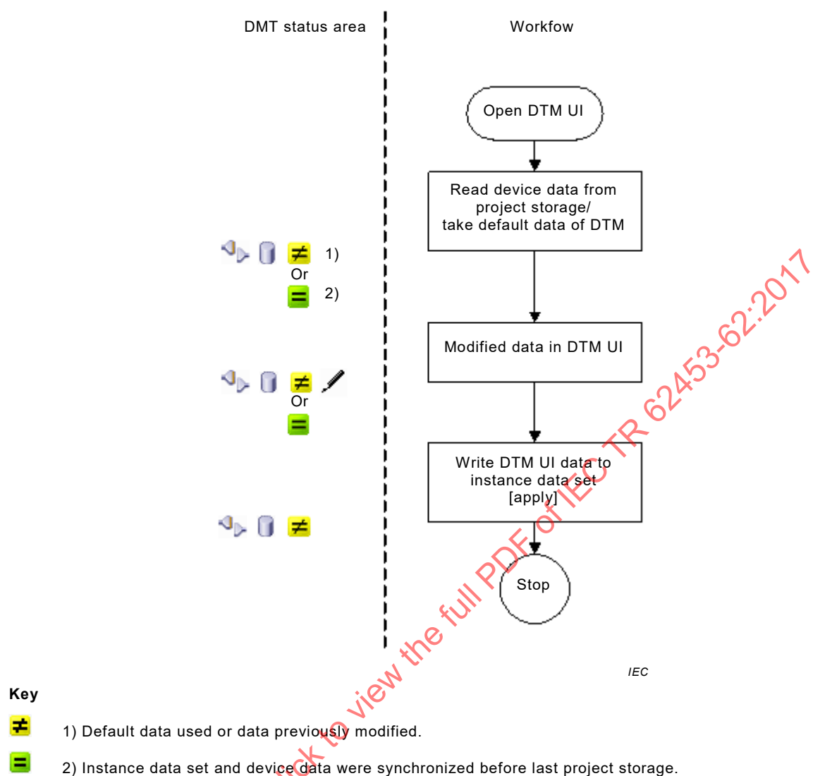
Figure 9 – Parameterize device offline
