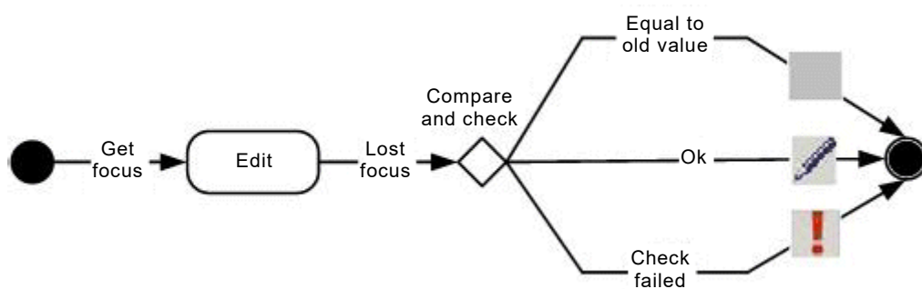
Figure 7 – State diagram: One Time Check
