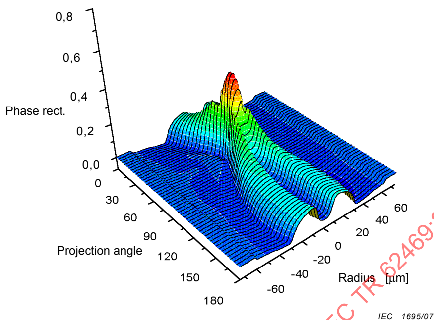
Figure 6 – Measured projected phases \delta(\gamma, \alpha) of a PM fibre for various projected angles as a function of fibre radius
