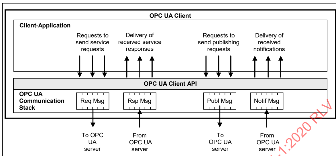
Figure 4 – OPC UA Client architecture
