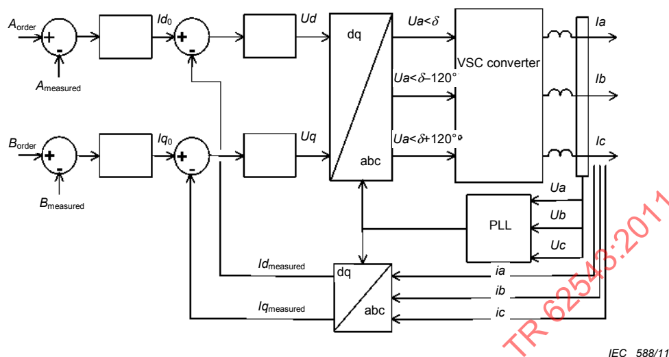
Figure 24 – Concept of vector control
