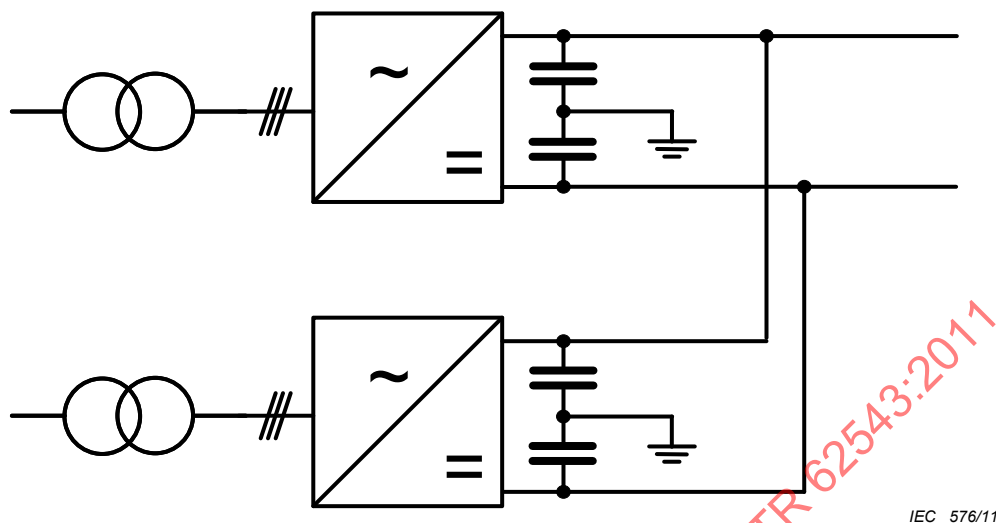
Figure 10 – Parallel connection of two converter units
