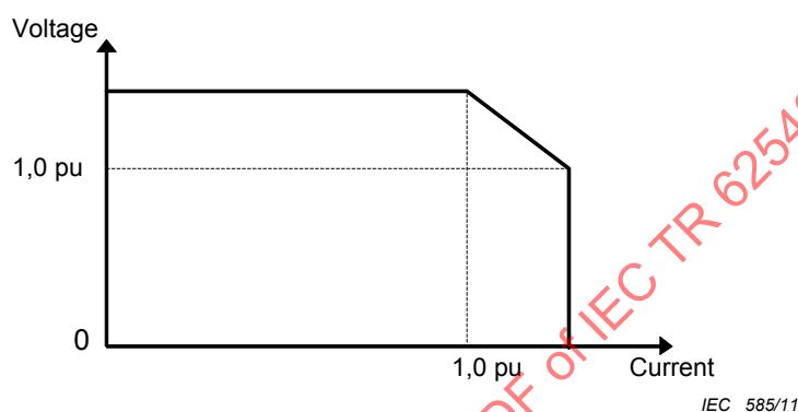
Figure 21 – Typical SSOA for the IGBT
