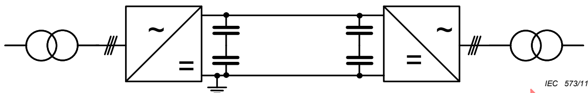
Figure 7 – VSC transmission with an asymmetrical monopole with metallic return
