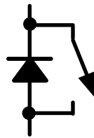
Figure 11 – Symbol of a controllable switch and associated free-wheeling diode
