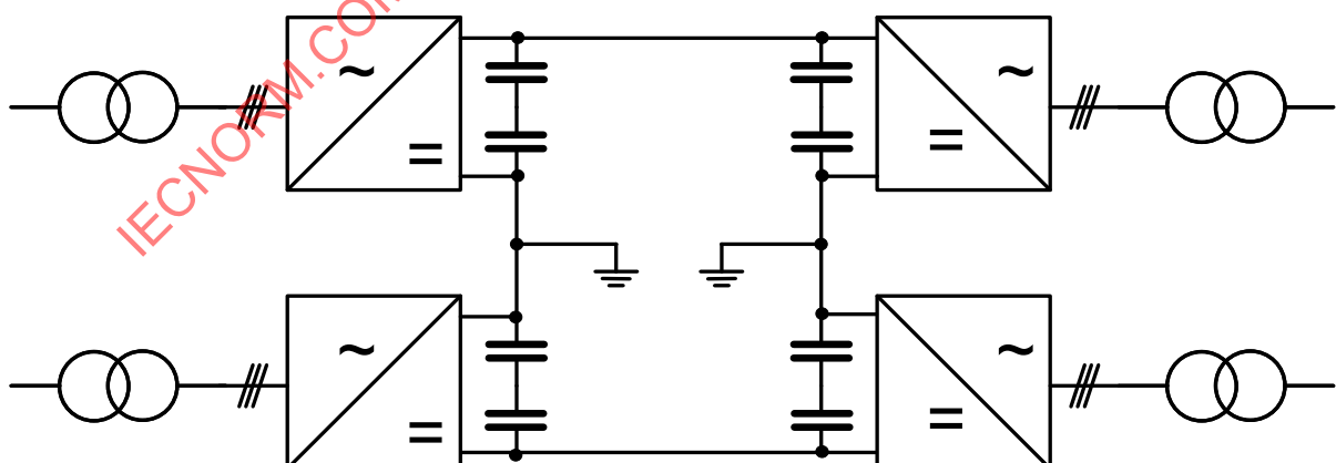
Figure 9 – VSC transmission in bipolar configuration
