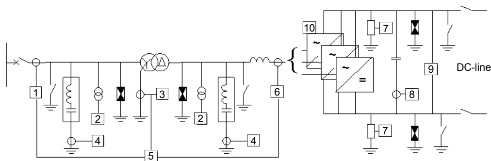
Figure 28 – Protection concept of a VSC substation
