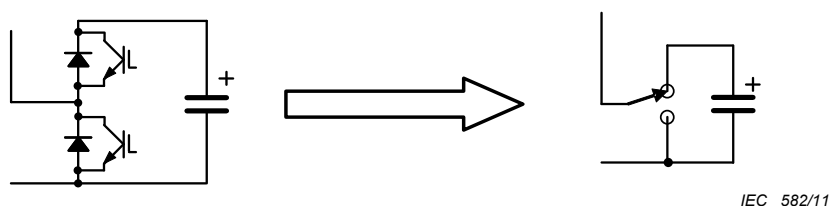
Figure 18 – VSC valve level arrangement and equivalent circuit in MMC topology in half-bridge topology
