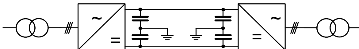
Figure 6 – VSC transmission with a symmetrical monopole
