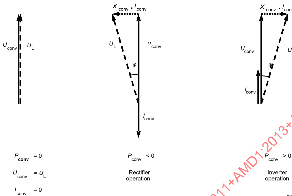
Figure 3 – The principle of active power control
