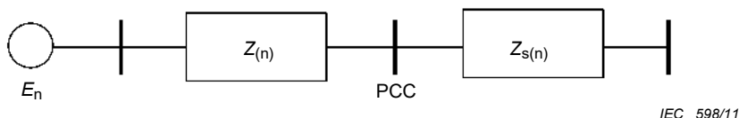
Figure 32 – Equivalent circuit at the PCC of the VSC
