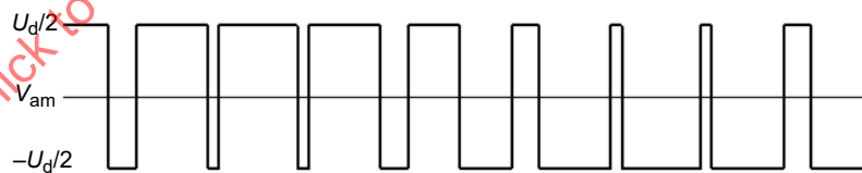
b) Phase a output voltage ( V_{am} )
