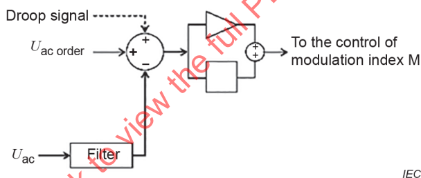
Figure 28 – AC voltage controller
