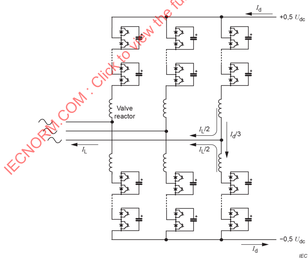
Figure 21 – Converter block arrangement with MMC topology in half-bridge topology
