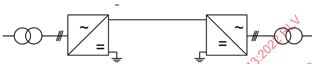
Figure 8 – VSC transmission with an asymmetrical monopole with earth return
