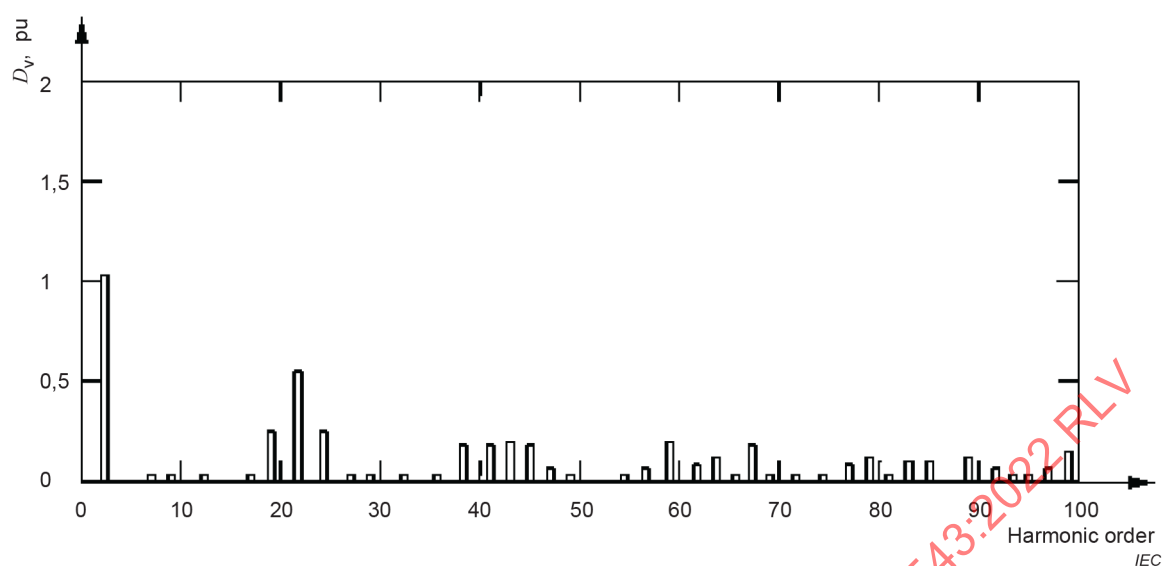
a) Phase-to-floating neutral voltage amplitude versus harmonic order
