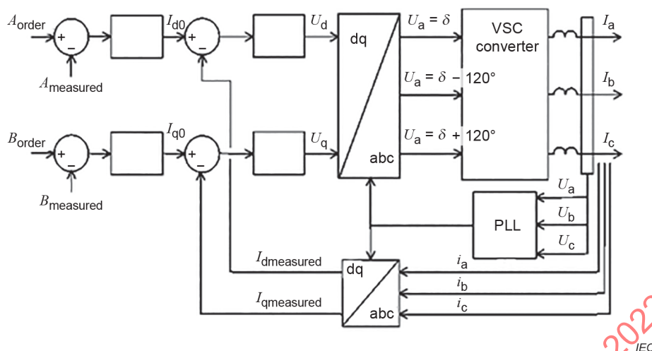
Figure 26 – Concept of vector control
