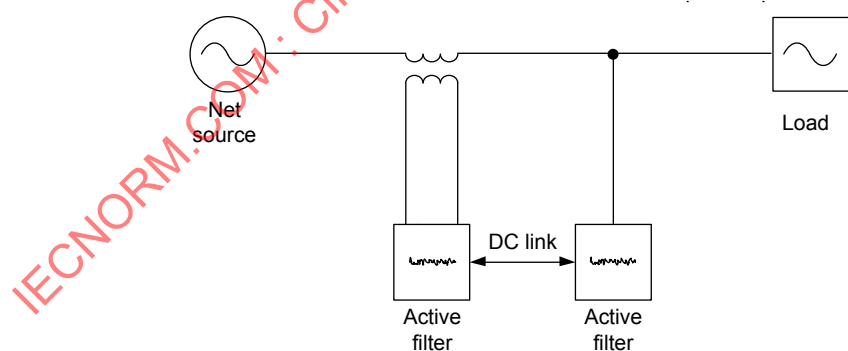
Figure 15 – Series and parallel connection
