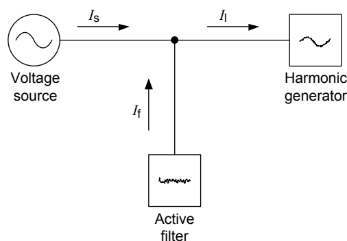
Figure 1 – Shunt connection IEC 1820/11
