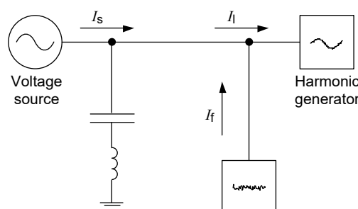
Figure 16 – Hybrid configuration
