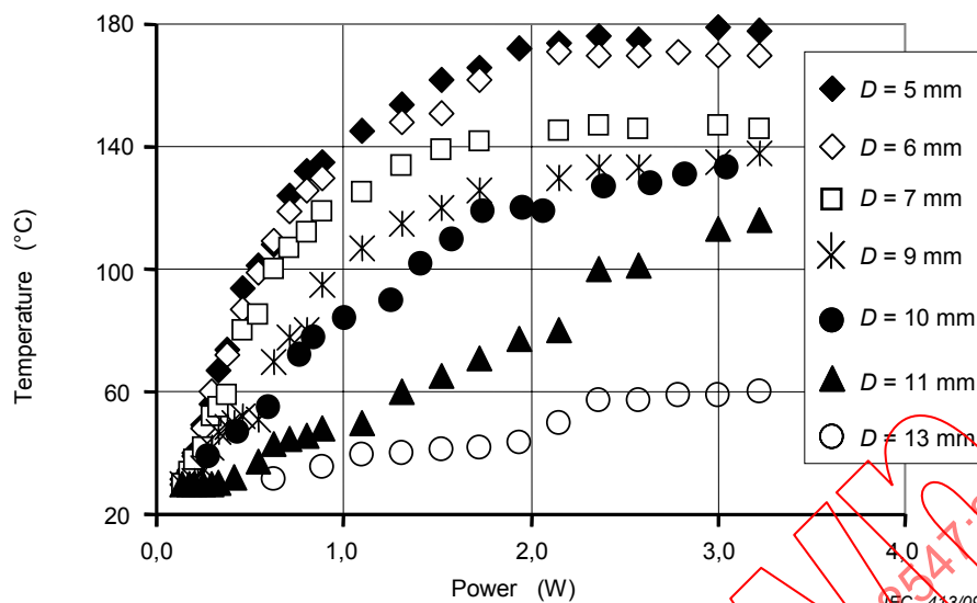
Figure 5 – Evolution of the coating equilibrium temperature as a function of launched power (see reference [10])
