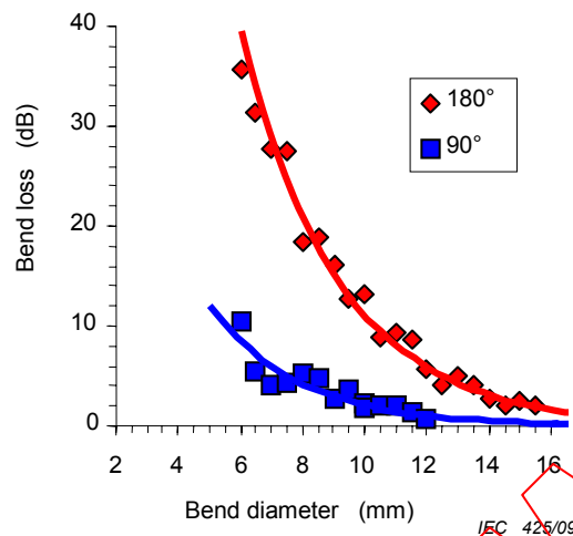
Figure A.11 – Bend loss performance at 180° (and 90° for reference) for fibre ‘D’ (see Clause A.7 for a full discussion)
