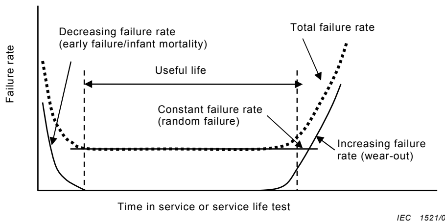
Figure 5 – “Bathtub” failure rate curve
