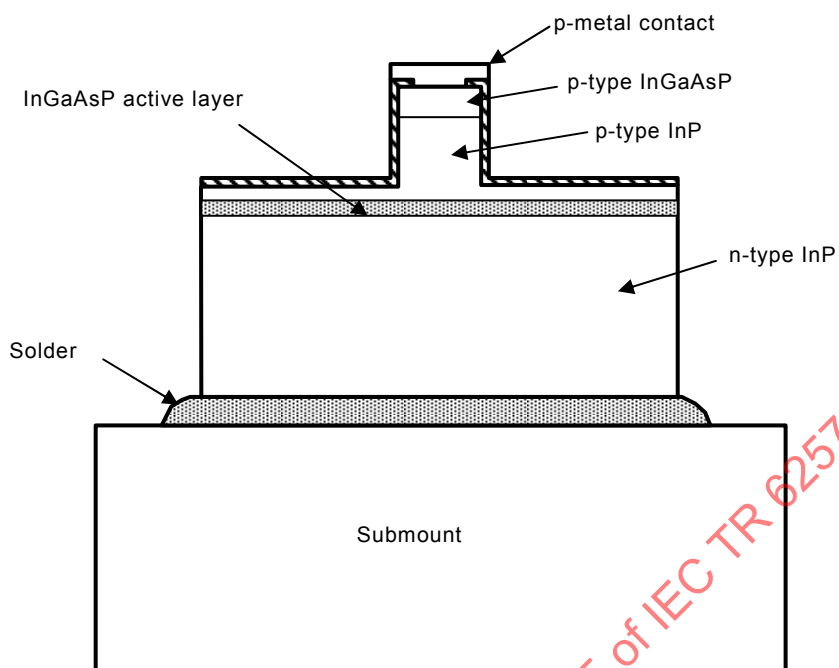
Figure 2a – Ridge waveguide type
