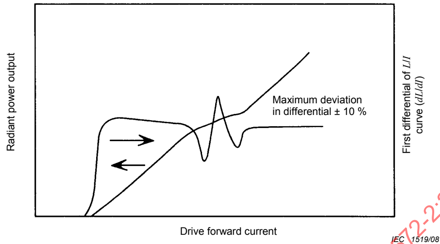
Figure 4a – Kinks in radiant power – forward current ( L/I ) curve
