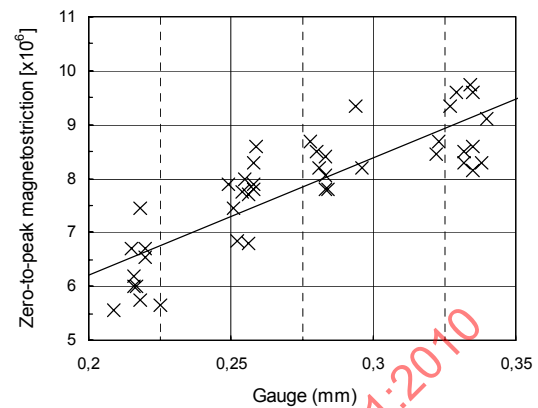
Figure 20 – Variation of maximum magnetostriction under compressive stress in conventional grain-oriented electrical steel at 1,5 T, 50 Hz [20]
