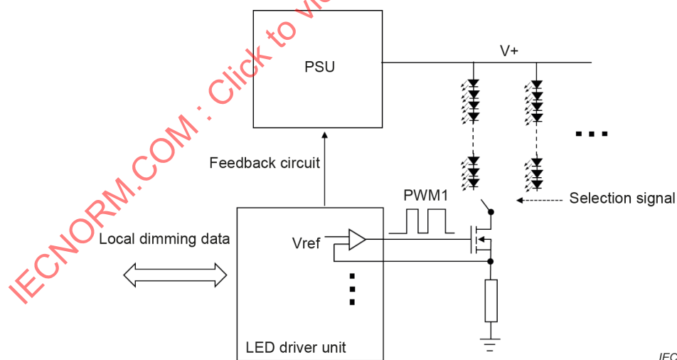
Figure 8 – Example of common anode mode LED backlight
