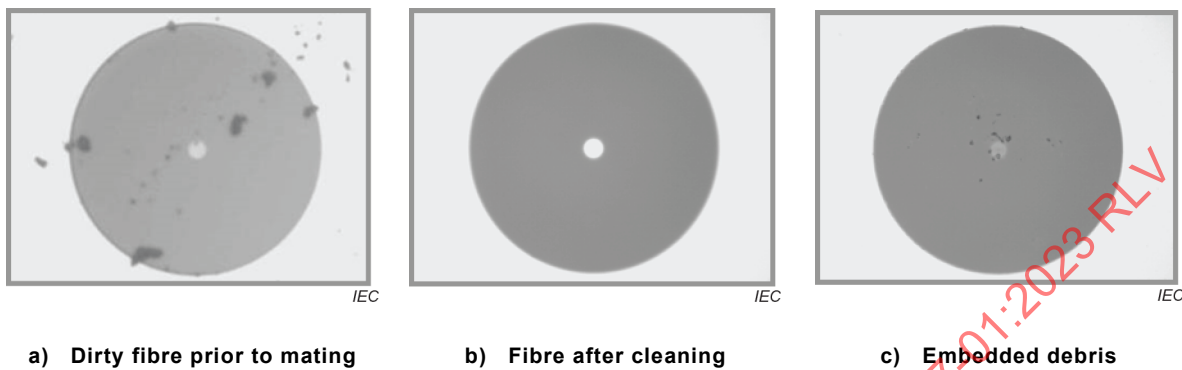
Figure B.5 – Permanent damage due to contamination
