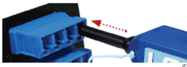
Figure 12 – Cleaning ports using a pen type cleaner
