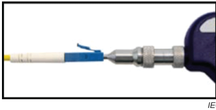
a) Fibre microscope for a plug
