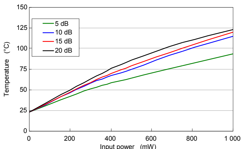
Figure 2 – Split sleeve out-surface temperature measurement results on high-power input condition for the SC plug style attenuators by Yamaguchi et al.
