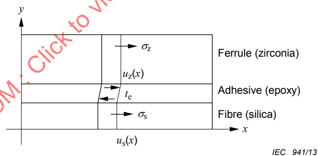
Figure 15 – Thermal stress simulation model for three layers of zirconia, epoxy and silica
