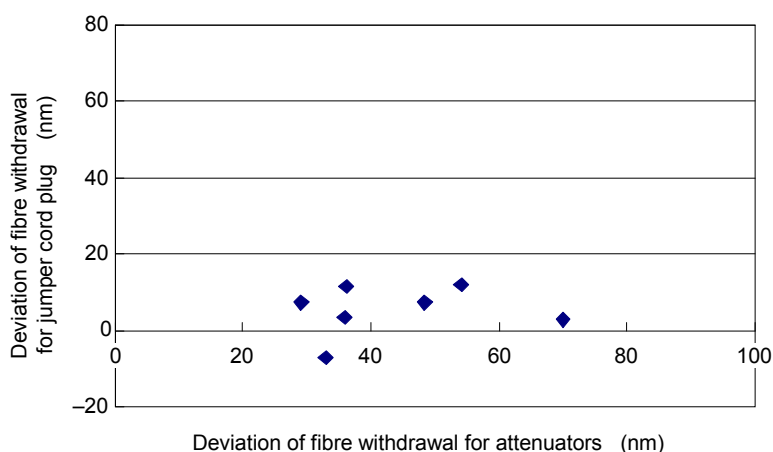
Figure 9 – Distribution diagram of the optical fibre withdrawal of both the optical attenuator and the optical connector
