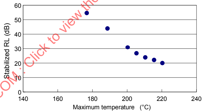
Figure 13 – Relationship between the maximum internal temperature and return loss stabilization point of the sample tested with various test temperatures and input powers (sample no. ATT44/JC35)
