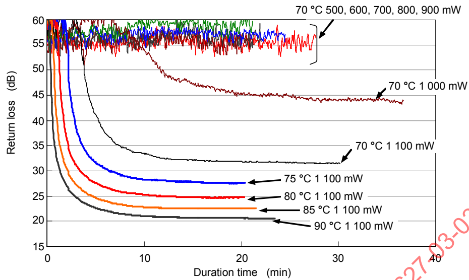
Figure 12 – Return loss decreasing curve in the tests with various test temperatures and input powers (sample no. ATT44/JC35)
