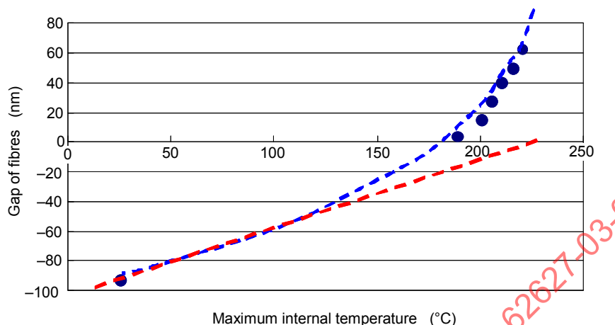
Figure 16 – Result of thermal distortion simulation and relationship between the sample maximum internal temperature and the gap
