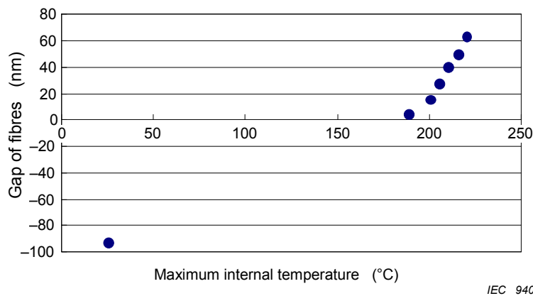
Figure 14 – Relationship between the maximum internal temperature and the gap at stabilization of return loss of the sample tested with various test temperature and input powers (sample no. ATT44/JC35)
