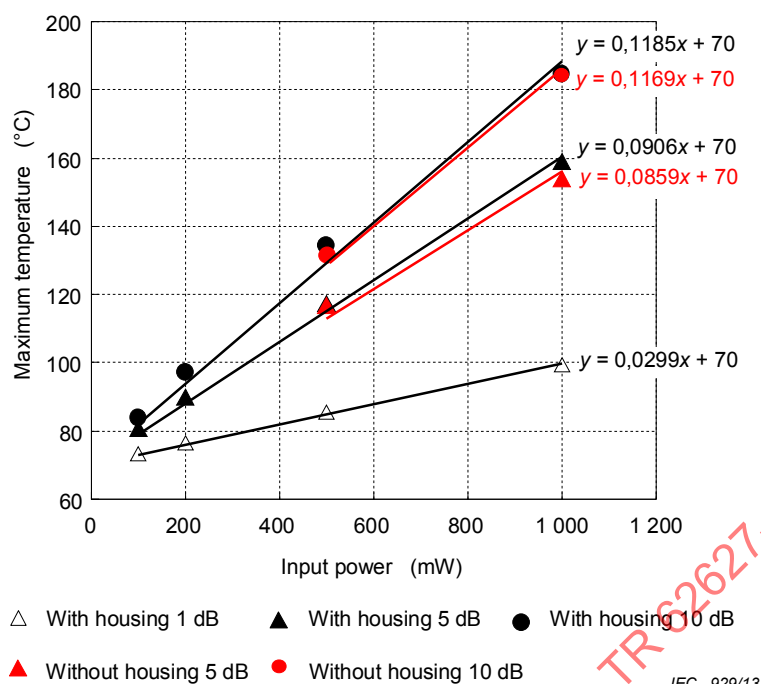
Figure 3 – Input-power dependency of split sleeve outer surface temperature of the SC plug style optical attenuator without housing
