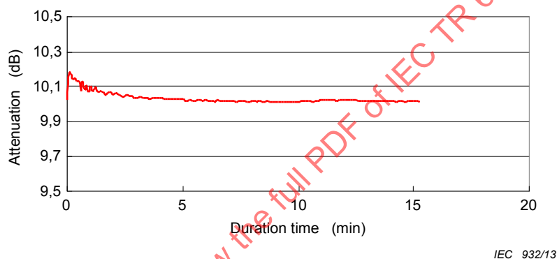
Figure 6 – High-power input test results of optical attenuator
