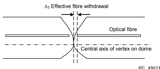
Figure 4 – Sample of design – Worst-case endface conditions
