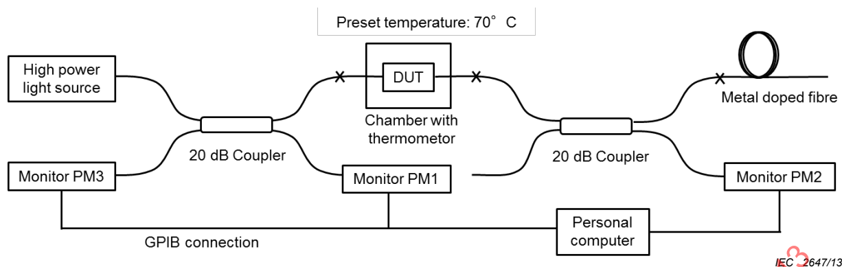
Figure 1 – Test set-up of high power step-stress test (example)
