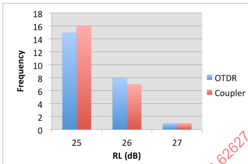
Figure 5 – RL random mated connectors, \lambda=1,300 nm [7]
