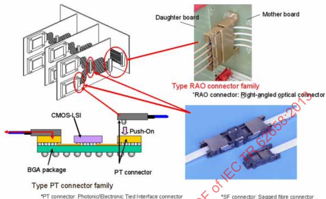
Figure 8 – Classification of optical circuit board connectors
