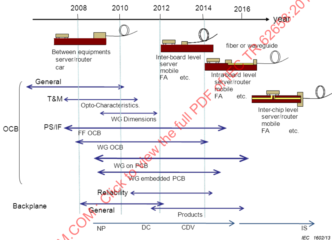
Figure 12 – Standardization roadmap of optical circuit board and its related optical packaging
