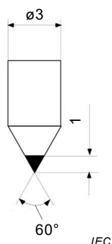
Figure A.9 – ø3 mm ceramic nail with Ni tip
