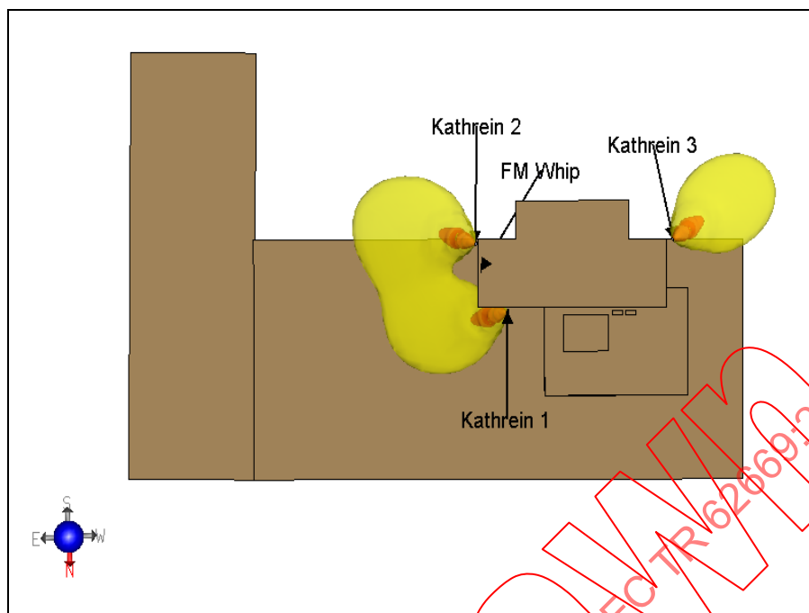
Figure 5.1.3: Top view of exclusion zones and building.
