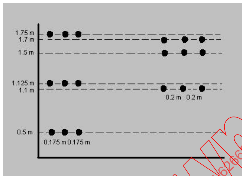
Figure 6: Example of the 9-points spatial averaging scheme as per Safety Code 6 and as Annex I of the IEC 62232
