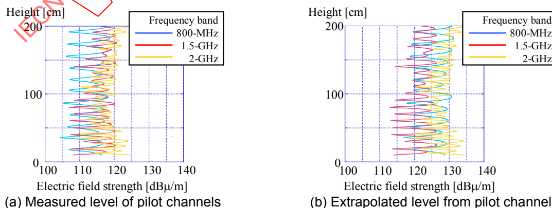
Figure 8. Electric field strength at just under antenna.
