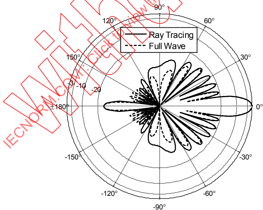
Figure 11.4: Vertical far-field radiation pattern comparison
