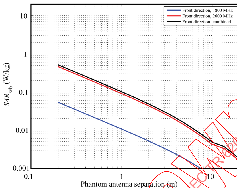
Figure 4: Whole-body SAR as function of separation distance.
