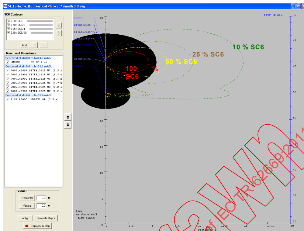
Figure 8: % of SC-6 compliance contours at ground level, at a height of 30 m ASL
