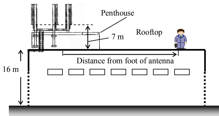
Figure 3.1.4.1 Antenna system of mobile base station installed on building roof-top
