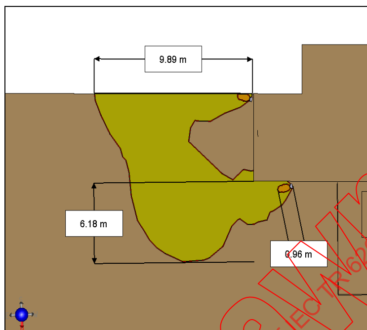
Figure 5.1.5: Top view - public and occupational caution lines surrounding antennas Kathrein 1 and 2.
