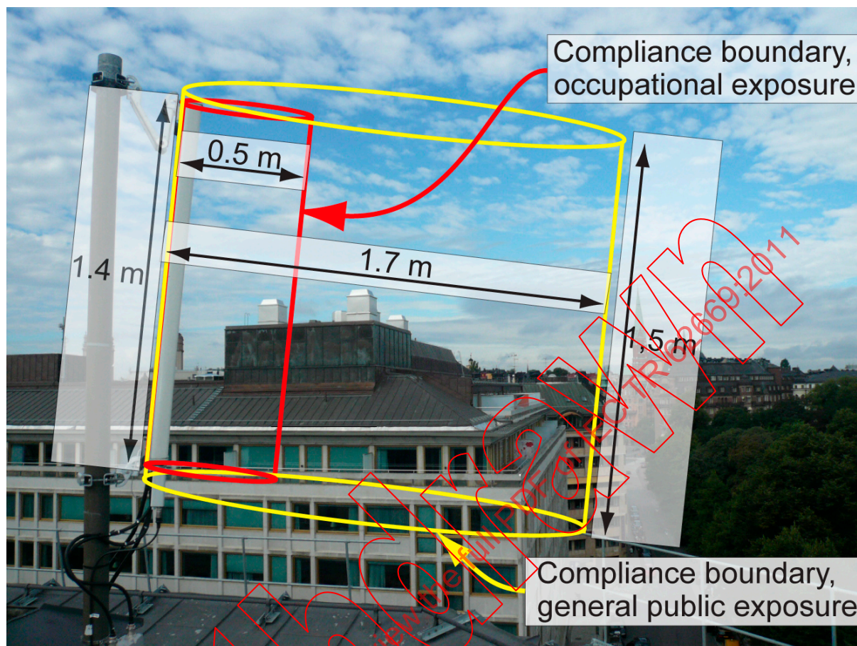
Figure 5: Base station antenna subject to assessment with calculated compliance boundaries (adult RF exposure).
