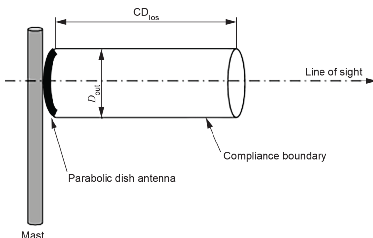
Figure 35 – Cylindrical shape RF compliance boundary
