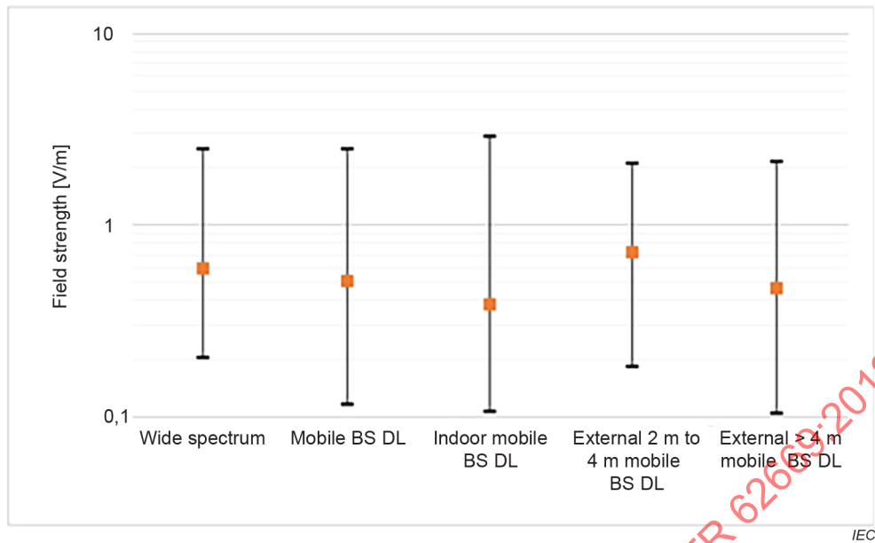
Figure D.9 – Results of the measurements around the selected sites
