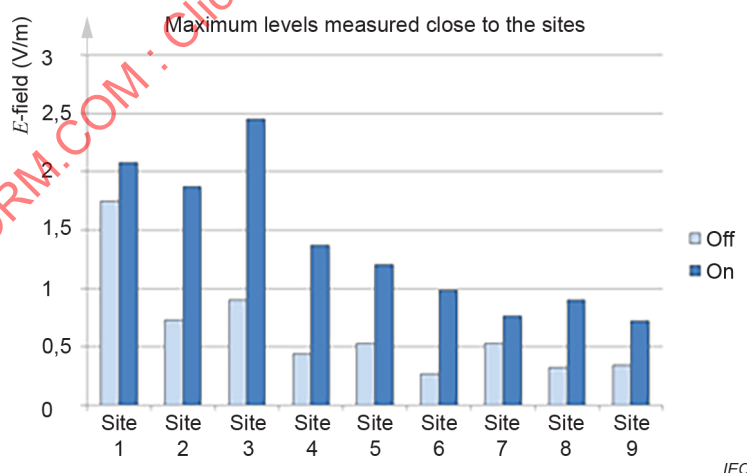
Figure D.2 – Maximum global E -field values measured in close proximity to the sites
