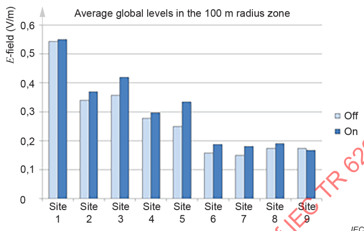
Figure D.1 – Mean value of E -field measurements with broadband equipment at intermediate points for each site
