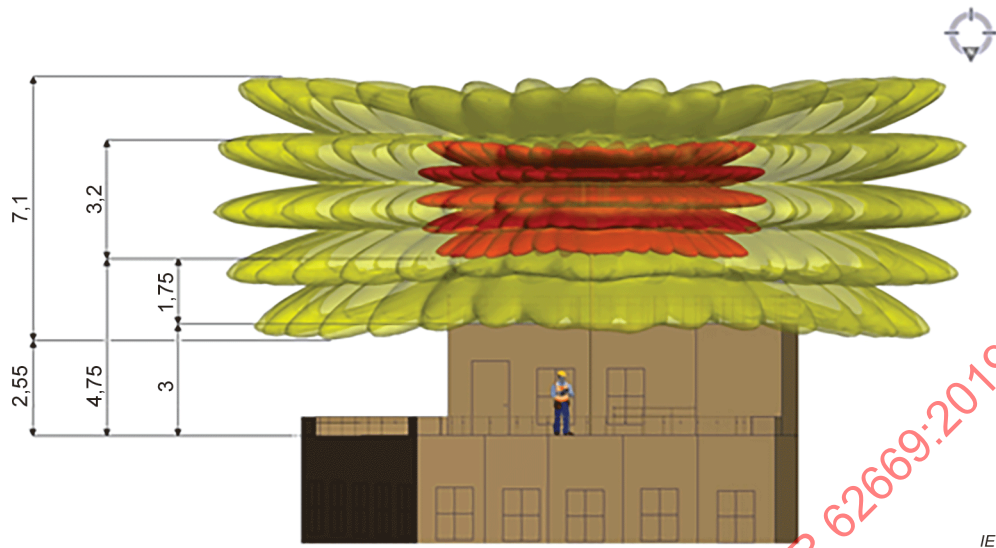
Figure 28 – Side view of the exclusion zones (red: occupational, yellow: general public)
