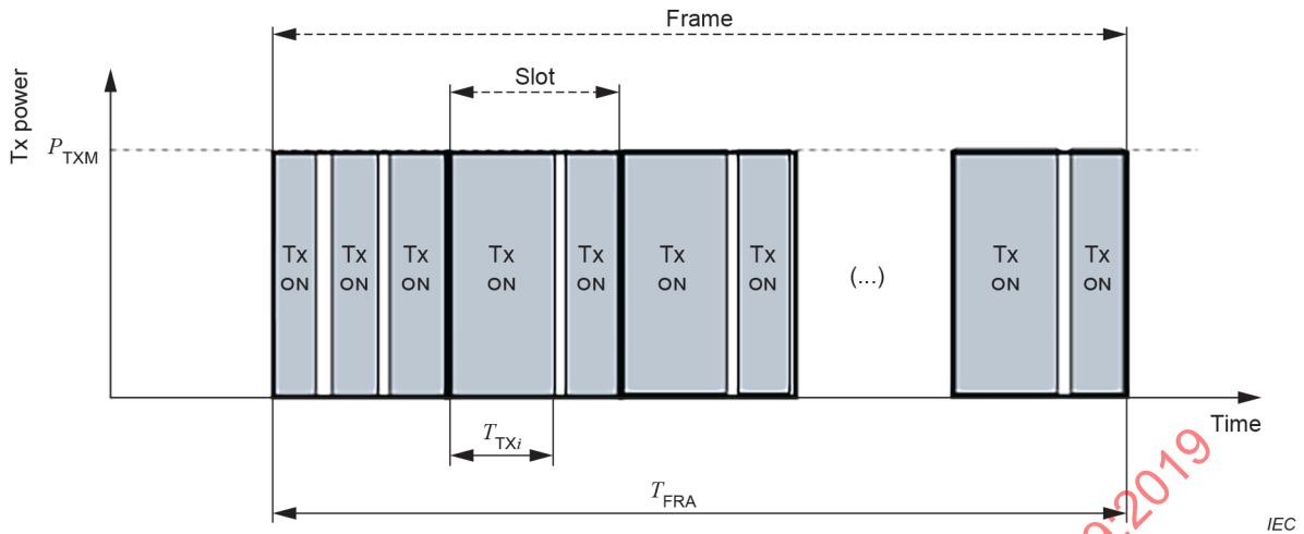
Figure 15 – Generic structure of a base station transmitted RF signal frame
