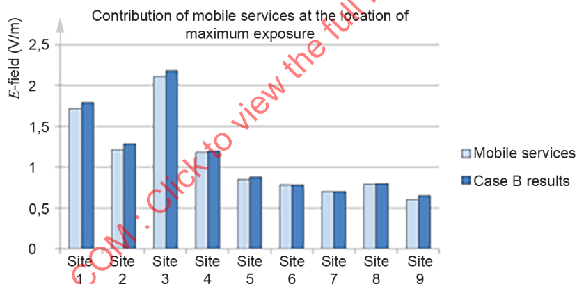
Figure D.4 – Contribution of mobile services compared to Case B results
