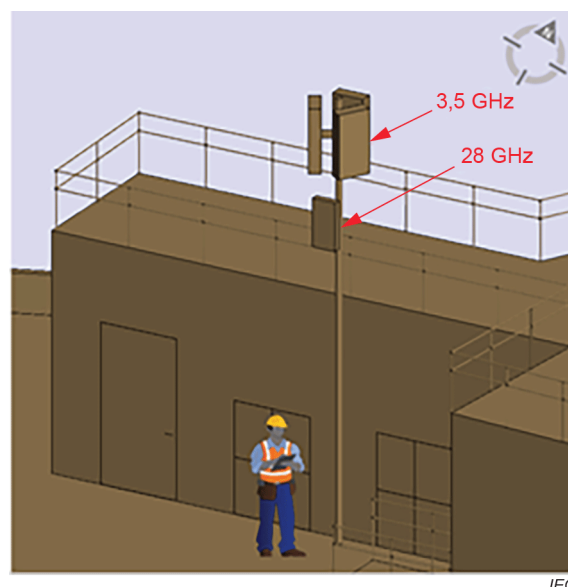
Figure 26 – Outline of the 5G site
