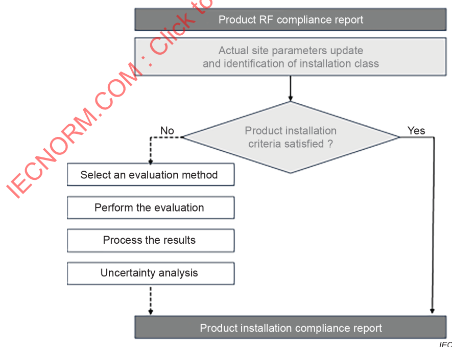
Figure 4 – Simplified process for product installation compliance applicable to small cells
