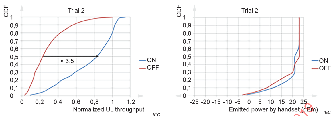
Figure D.7 – Cumulative distribution function of the upload throughput on Trial 2 normalized by the maximum value measured on each site when the small cells are off (left) and of the transmitted power by the handset (right)
