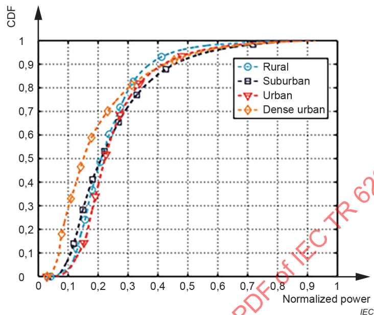
Figure 12 – Empirical CDFs of transmitted power (normalized) for different environments in 3G network in India [31]
