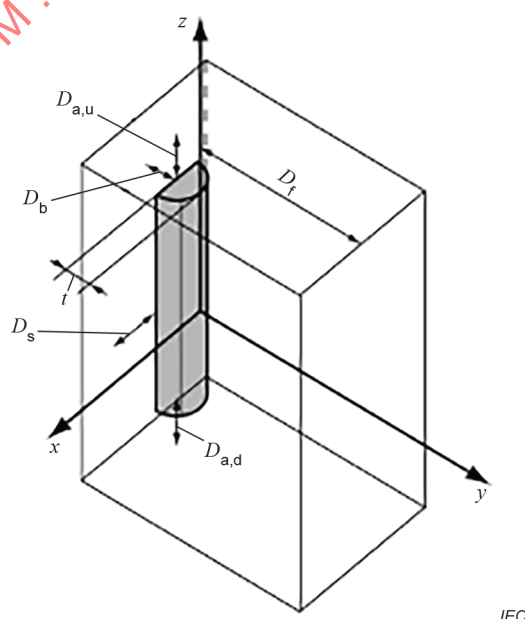
Figure 25 – Box-shaped RF compliance boundary
