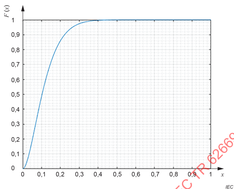
Figure 22 – CDF of the reference Beta distribution used to assess power combination factors
