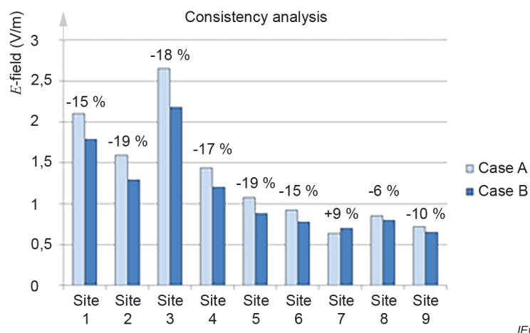
Figure D.3 – Consistency analysis between Case A and Case B (without extrapolation) results
