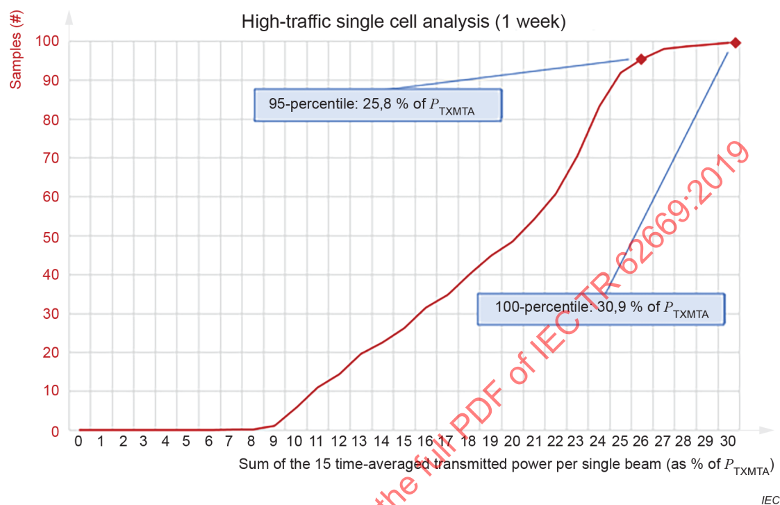
Figure 21 – CDF in high-traffic conditions (experiment #5)
