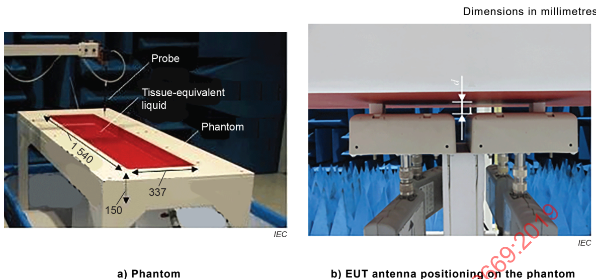
Figure B.1 – Views of the SAR measurement setup
