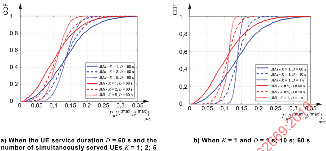
Figure 18 – CDF of the normalized transmitted power for both UMa and UMi
