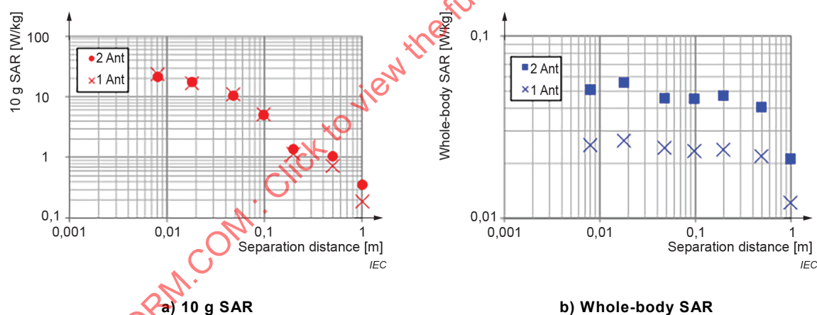
Figure B.2 – Characteristics of SAR of EUT antennas as a function of separation distance at 3,5 GHz
