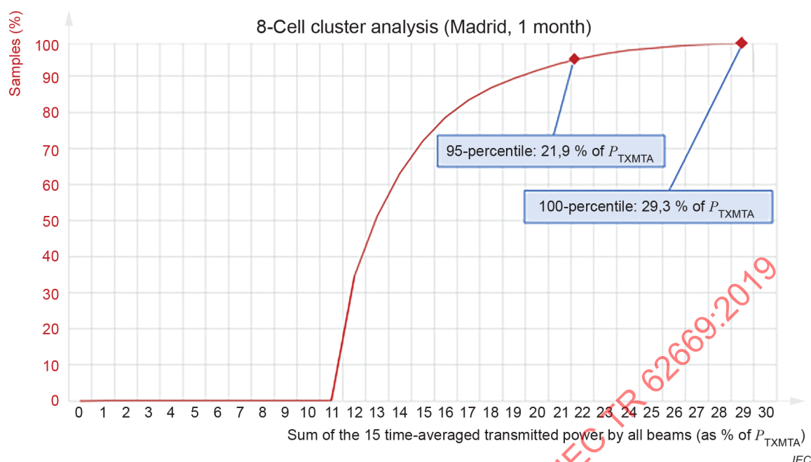
Figure 20 – CDF of measurement on 8-cell cluster (experiment #1)
