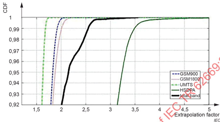
Figure 14 – Extrapolation factor of the power flux density S(t) of the different signals and the S_{\text{total}}(t) (all bands) with a sliding time averaging of 6 min applied to the measurements [27]
