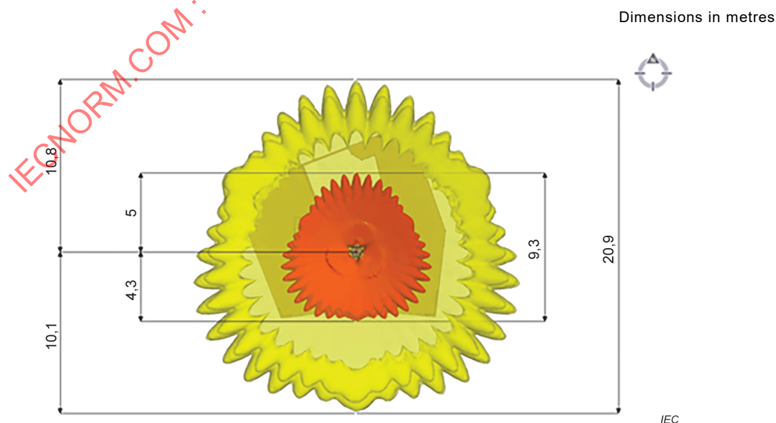
Figure 27 – Top view of the exclusion zones (red: occupational, yellow: general public)
