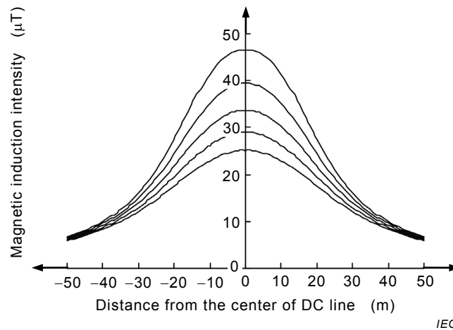
Figure 2 – Lateral profile of magnetic field on the ground of ±800 kV HVDC lines
