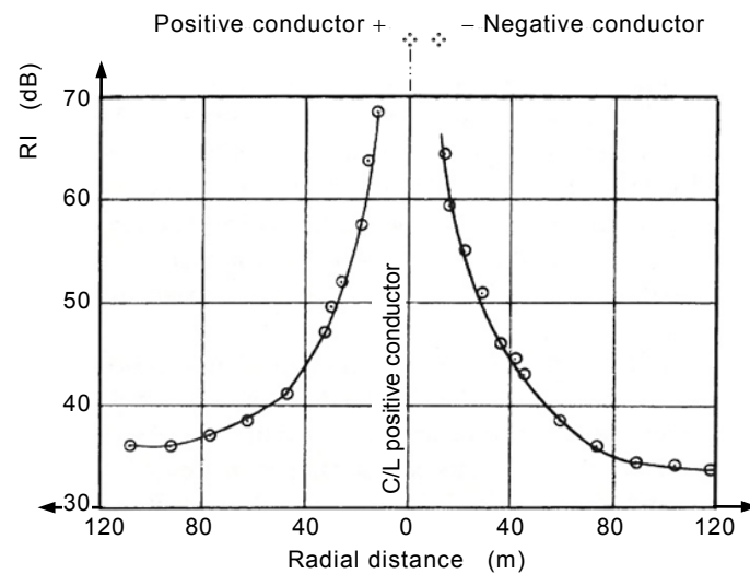
Figure B.2 – Typical RI lateral profile at \pm 600\text{kV} , 4 \times 30,5\text{ mm} conductor, 11,2\text{ m} pole spacing, 15,2\text{ m} average height [12]
