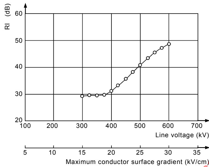
Figure B.4 – RI at 834kHz as a function of bipolar line voltage 4 × 30,5 mm conductor, 11,2 m pole spacing, 15,2 m average height
