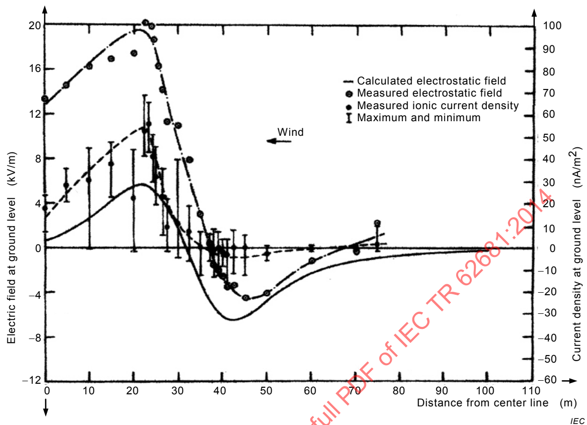
Figure A.1 – Electric field and ion current distributions for Manitoba Hydro \pm 450 kV Line [37]
