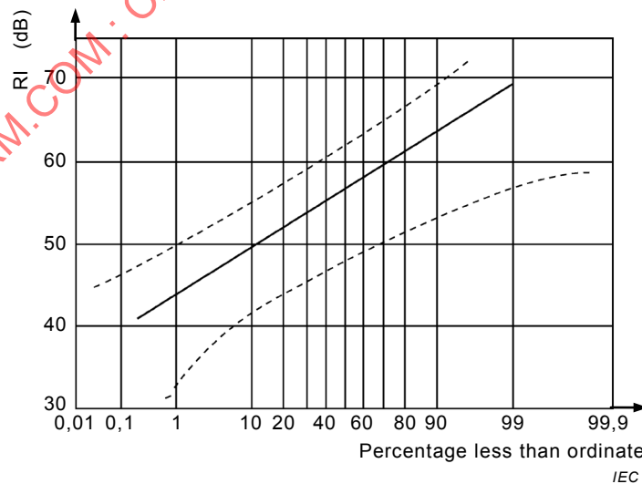
Figure B.5 – Percent cumulative distribution for fair weather, 2 × 46 mm, 18,3 m pole spacing, ±600 kV
