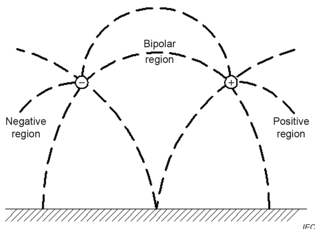
Figure 1 – Unipolar Monopolar and bipolar space charge regions of an HVDC transmission line [1]
