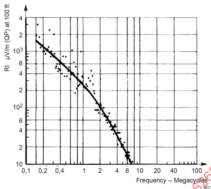
Figure B.10 – RI vs. frequency at \pm 400 kV [124]
