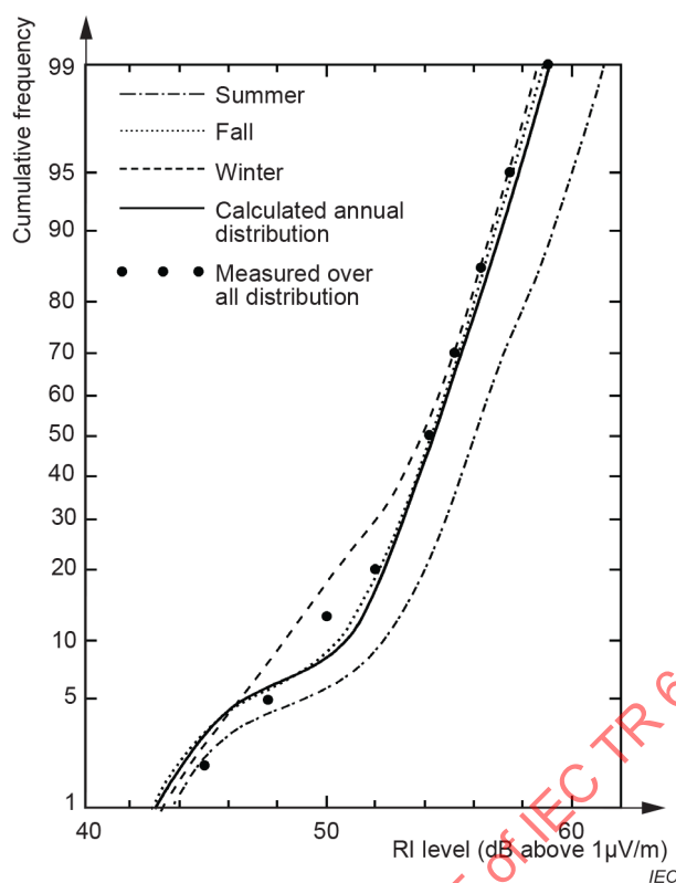
Figure B.11 – Cumulative distribution of RI measured at 15 m from the positive pole [125]
