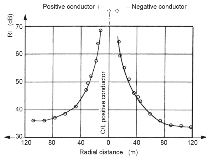
Figure B.2 – Typical RI lateral profile at \pm 600 kV, 4 \times 30,5 mm conductor, 11,2 m pole spacing, 15,2 m average height [14]
