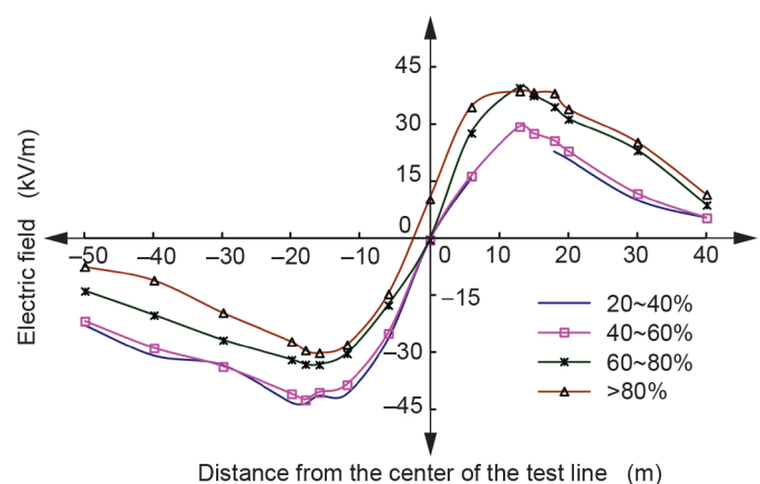
Figure A.4 – Test result for total electric field at different humidity [119]
