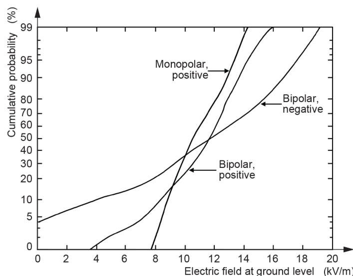
Figure A.2 – Cumulative distribution of electric field for Manitoba Hydro ±450 kV Line [39]
