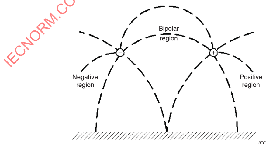
Figure 1 – Monopolar and bipolar space charge regions of an HVDC transmission line [1]
