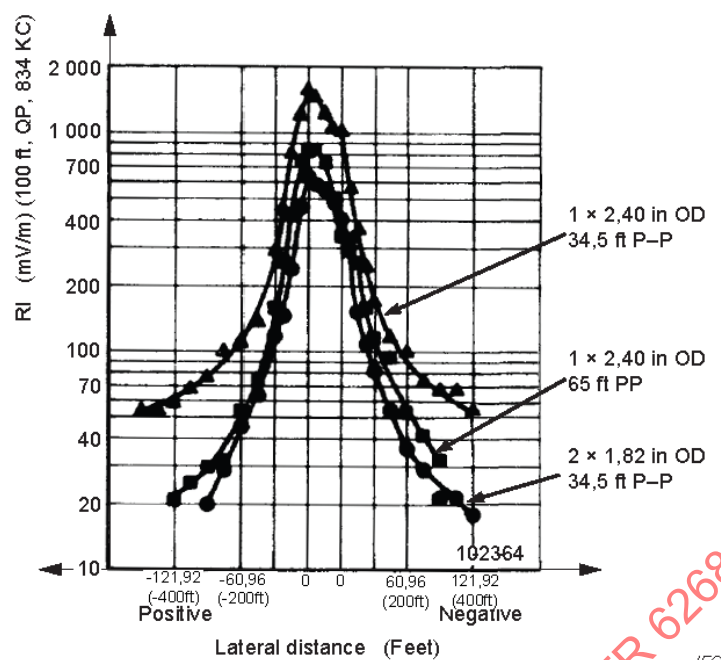
Figure B.3 – Simultaneous RI lateral, midspan, in clear weather and light wind for three configurations, bipolar \pm 400 kV [124]
