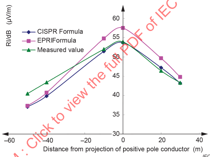
Figure B.14 – Comparison between calculation result and test result for RI lateral profile [119]
