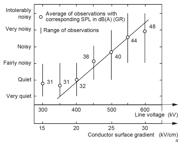
Figure 15 – Subjective evaluation of DC transmission line audible noise; OSU study 1975 [14]
