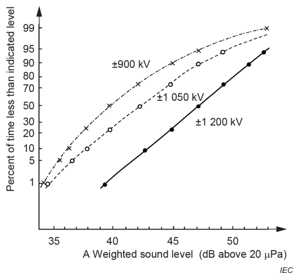
Figure C.1 – Examples of statistical distributions of fair weather audible noise. dB(A) measured at 27 m from line centre of a bipolar HVDC test line [16]
