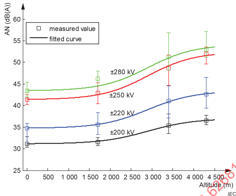
Figure C.2 – AN under the positive polar test lines varying with altitude
