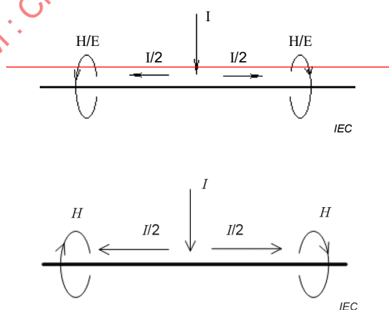
Figure 3 – The corona current I and radio interference magnetic field H
