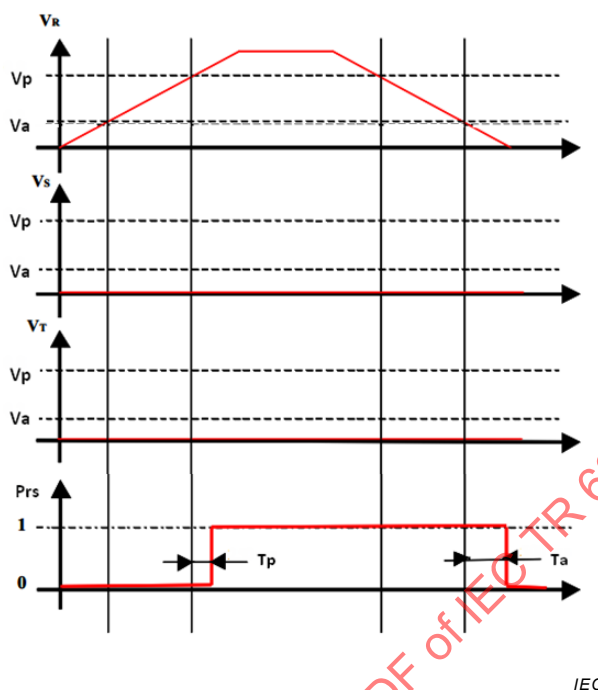
Figure 9 – Voltage presence/absence
