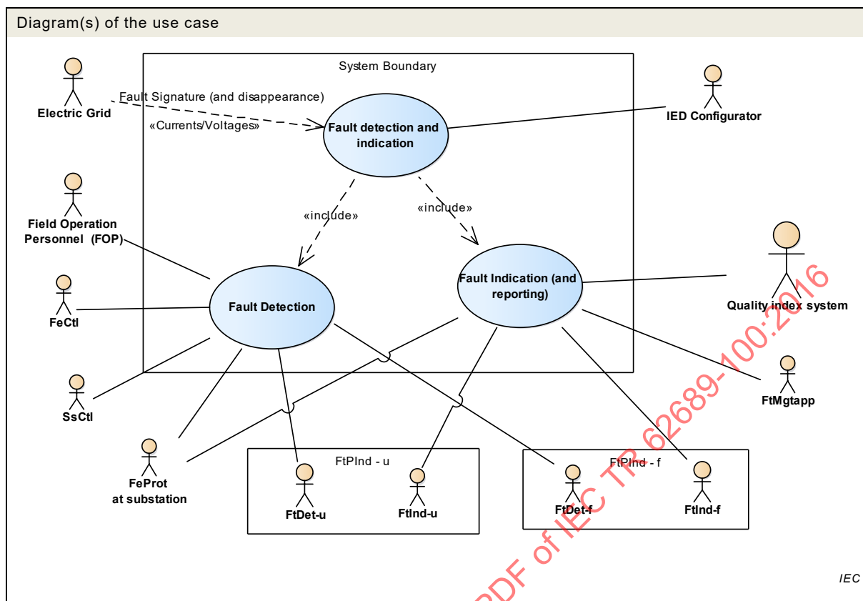
Figure 4 – Fault indication – Main use case
