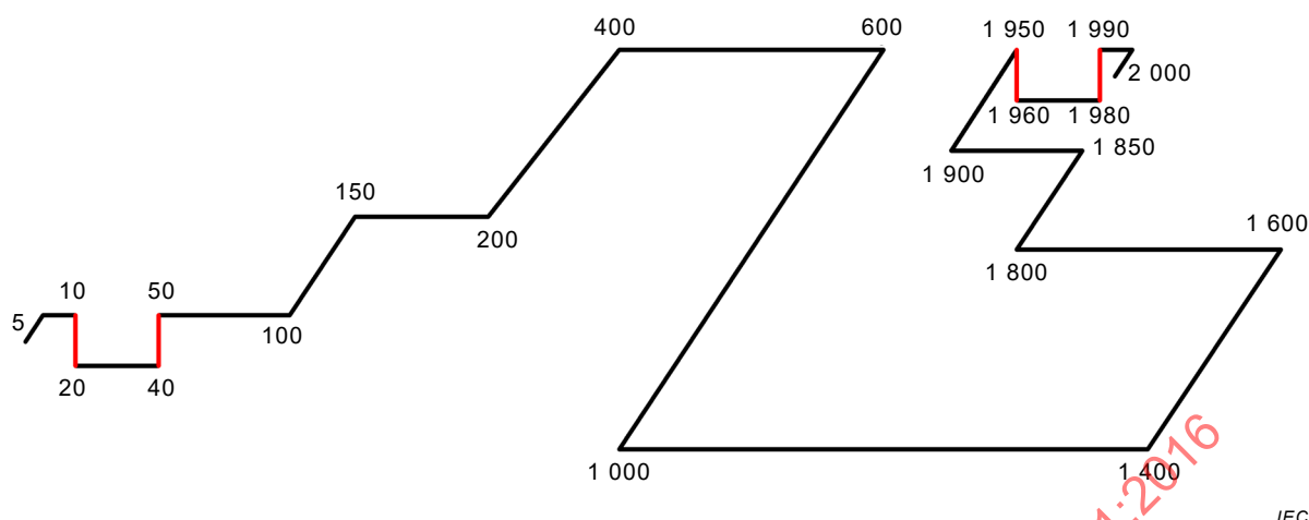
Figure 2 – Cable tension calculations (Equations (4) to (9))
