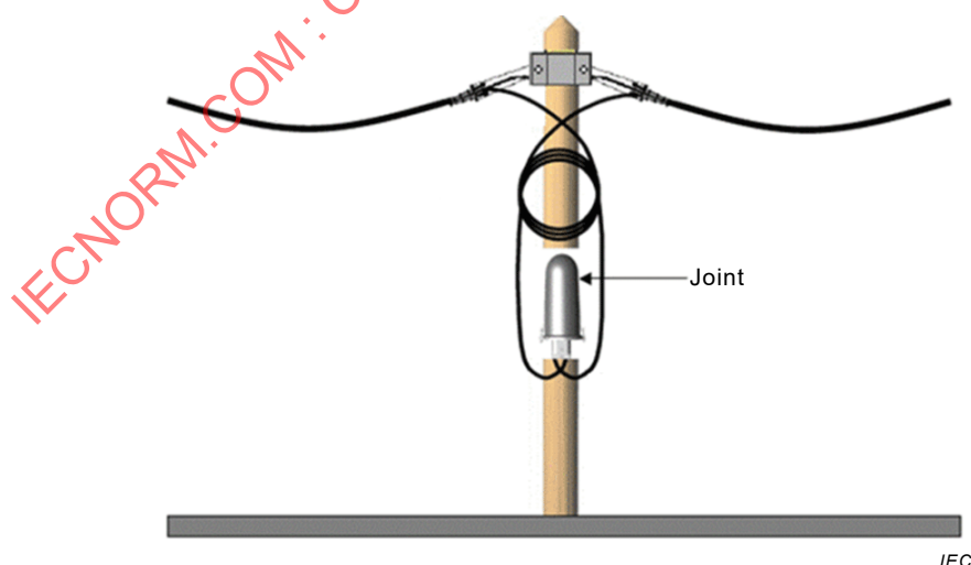
Figure 11 – Aerial cable joint point
