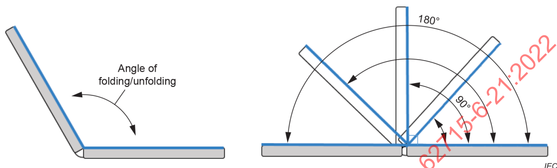
Figure 9 – Angle of folding and unfolding
