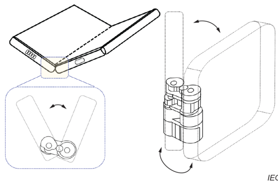
Figure 7 – General hinge structure
