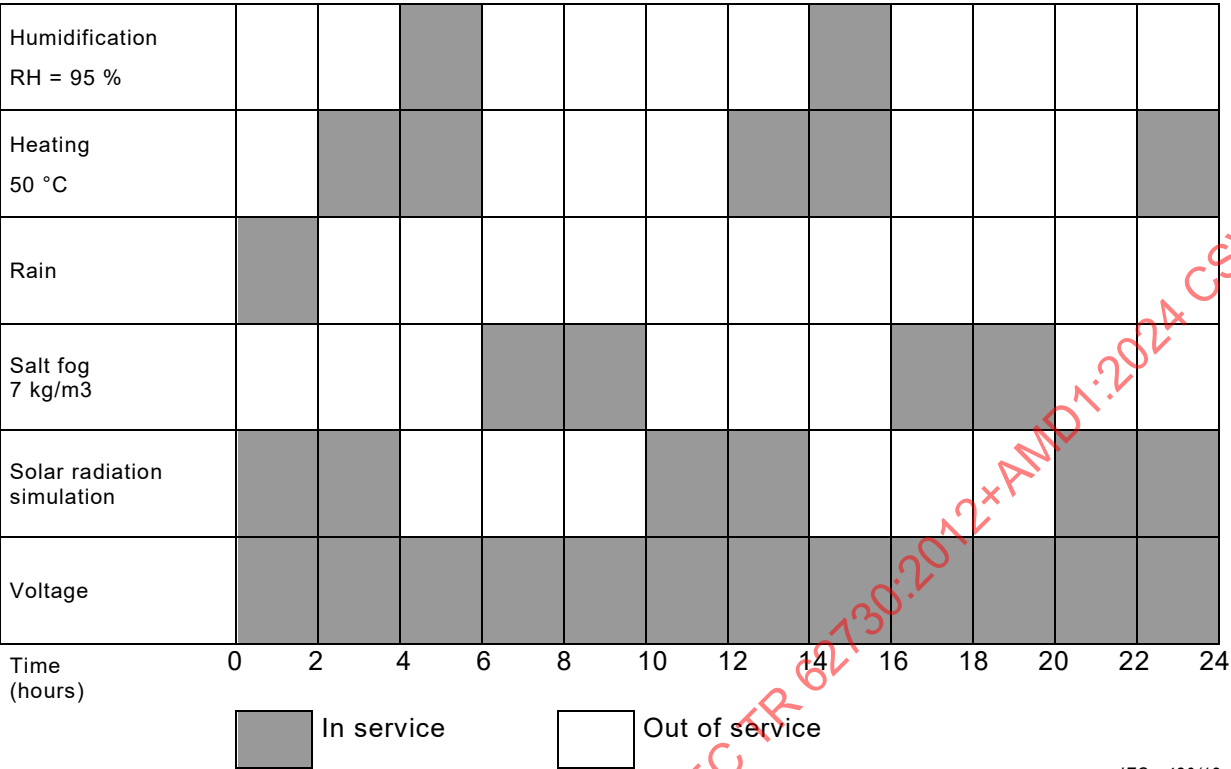
Figure 3 – Multiple stress cycle
