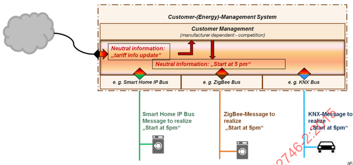
Figure 10 – Example of a mapping of messages
