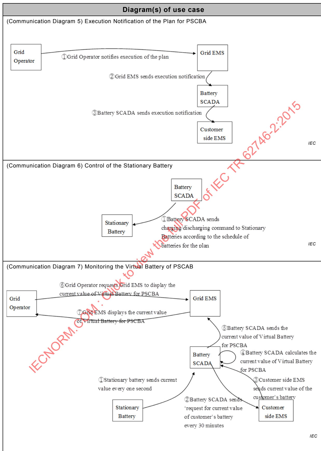
Figure A.25 – Use case diagram
