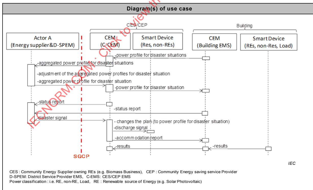
Figure A.27 – Sequence diagram
