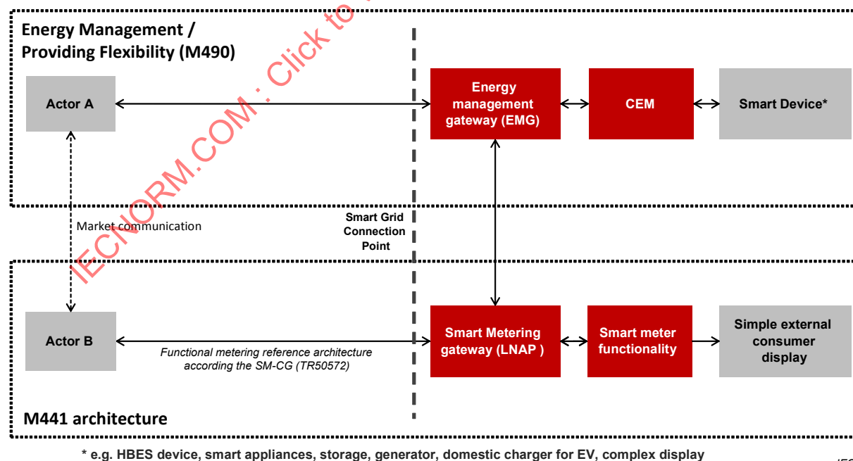
Figure A.20 – SG CG Architecture Model [9]
