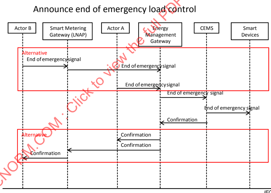
Figure A.30 – Sequence diagram
