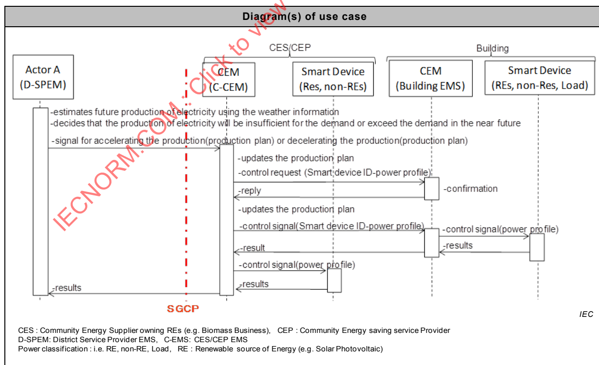
Figure A.26 – Sequence diagram
