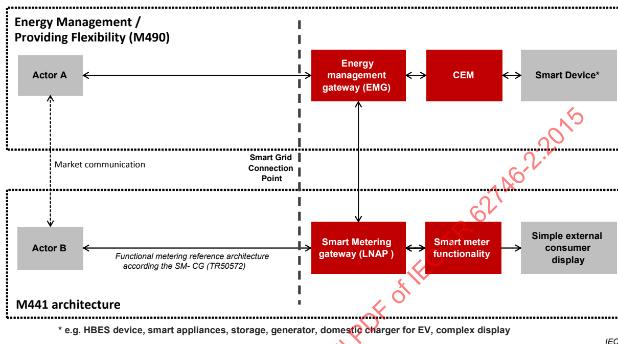
Figure A.4 – SG CG Architecture Model [9]
