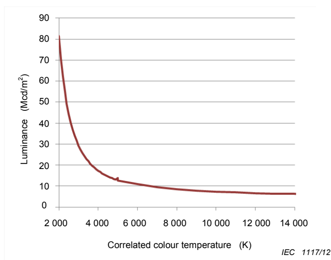
Figure 4 – Estimate of the luminance level where L_B = 10\,000\text{ W}/(\text{m}^2\cdot\text{sr}) , border between RG1 ( t_{\max} > 100\text{ s} ) and RG2 ( t_{\max} < 100\text{ s} ) in the large source regime, as a function of CCT
