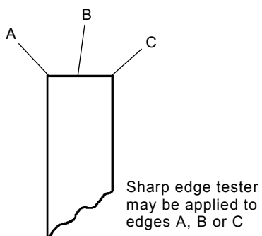
Figure 5 – Test Procedure
