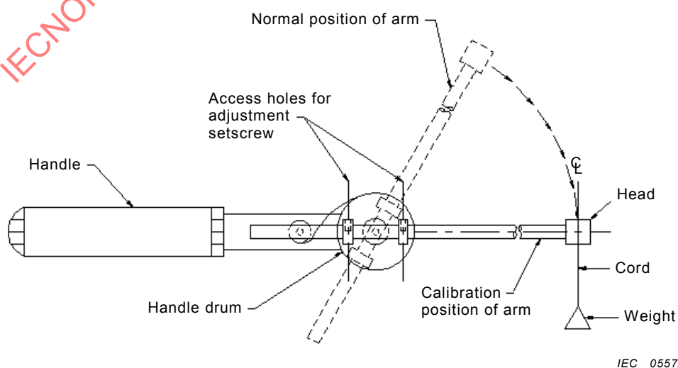
Figure 3 – Typical calibration procedure
