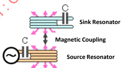
Figure 7 – Magnetic resonance
