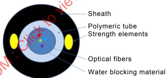
Figure 18 – Lashed cable
