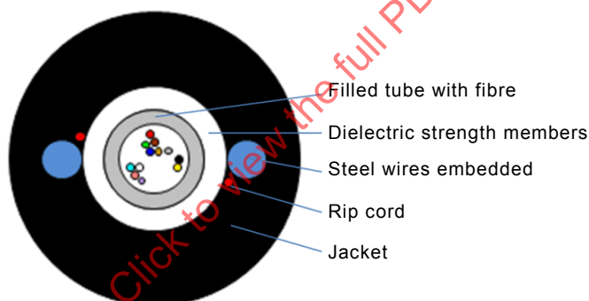
Figure 14 – Self-supporting aerial cable with non concentrically-arranged strength members
