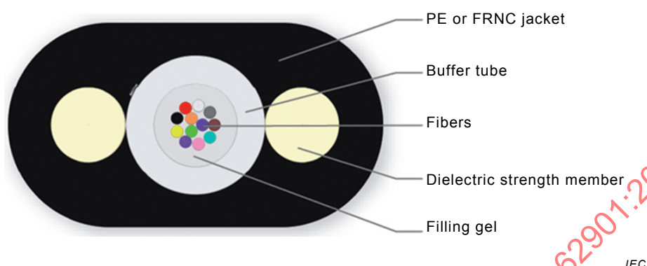
Figure 15 – Flat self-supporting aerial cable with strength members on both sides
