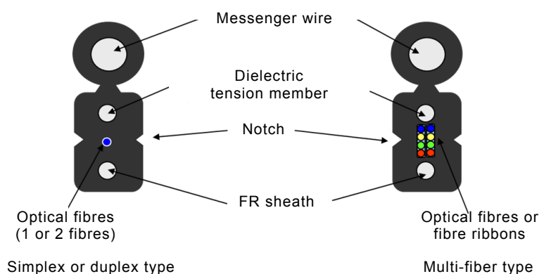
Figure 16 – Rectangular design with one integrated messenger wire and strength members
