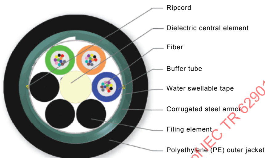
Figure 8 – Tape armored cable
