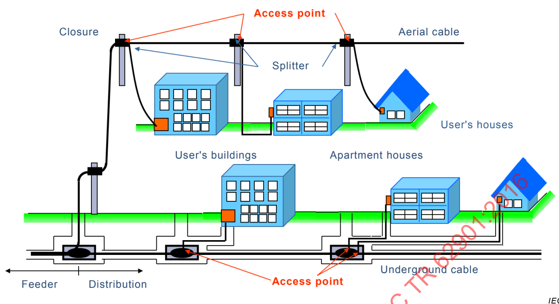
Figure 1 – Configuration of a typical FTTH network
