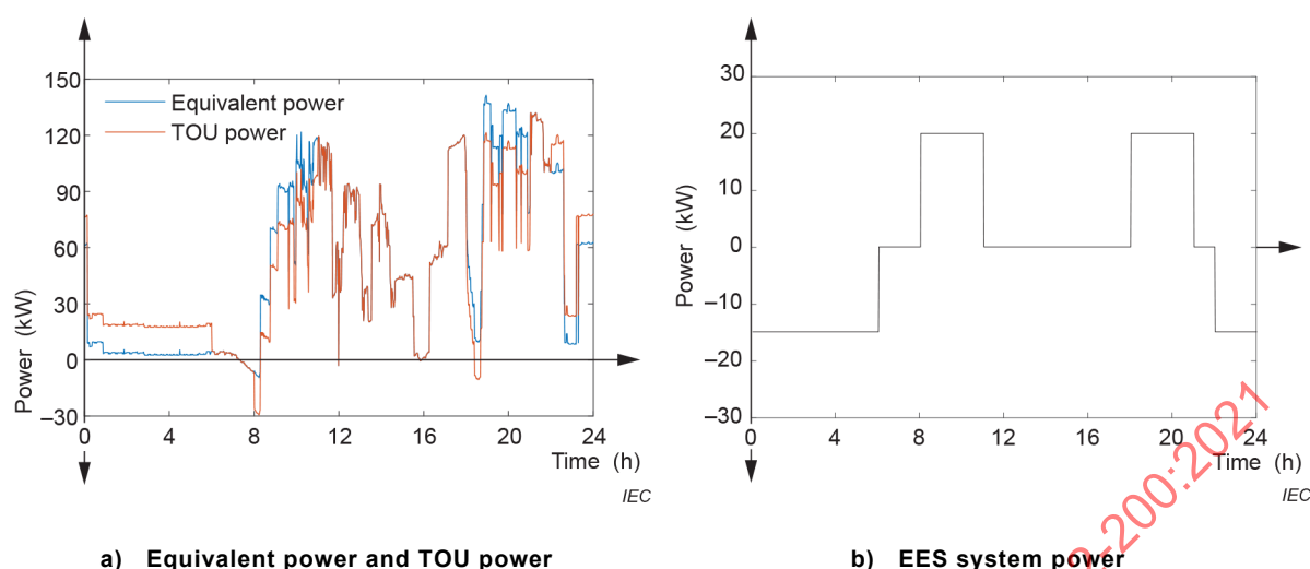
Figure 13 – Operating power in the TOU price arbitrage mode for the case of a commercial charging station based on common AC bus
