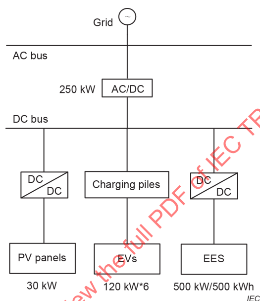
Figure 2 – System structure for the case of a commercial PV-EES-EV charging station based on common DC bus
