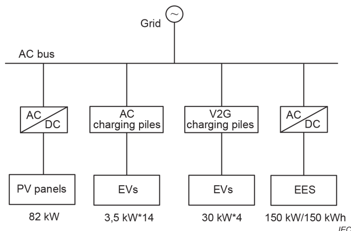
Figure 9 – System structure for the case of a commercial PV-EES-EV charging station based on common AC bus
