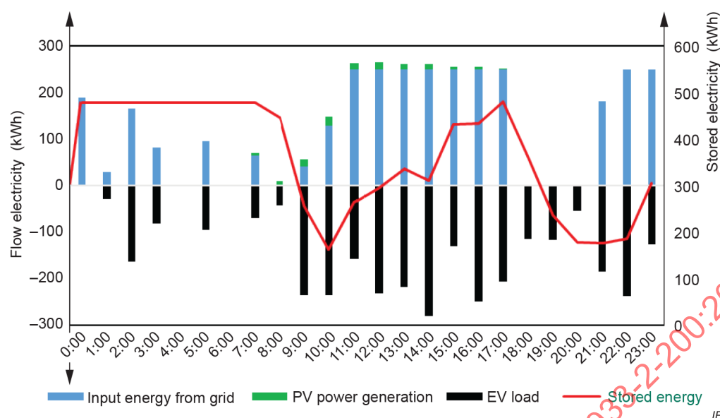
Figure 8 – Daily electricity flow for the case of a commercial charging station based on common DC bus
