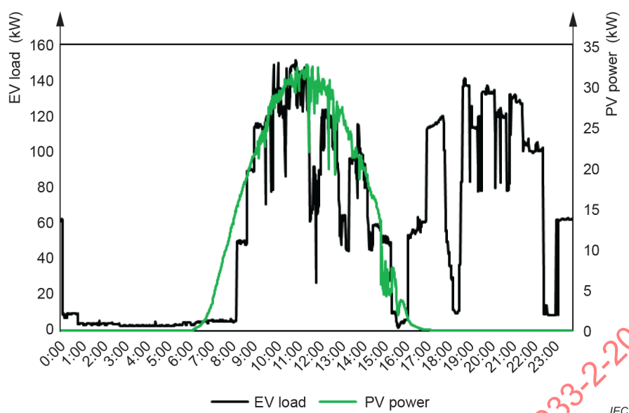
Figure 10 – EV load and PV power for the case of a commercial charging station based on common AC bus
