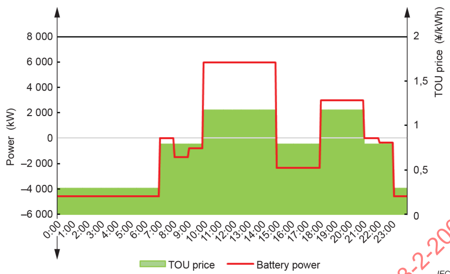
Figure 20 – Operating power in TOU price arbitrage mode for the case of a business charging station based on common DC bus
