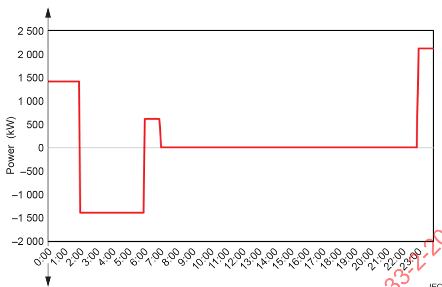
Figure 21 – Operating power in demand response mode for the case of a business charging station based on common DC bus
