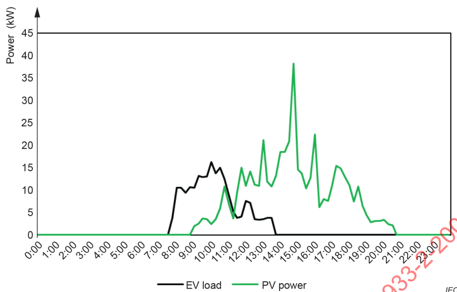
Figure 26 – EV load and PV power for the case of a business charging station based on common AC bus
