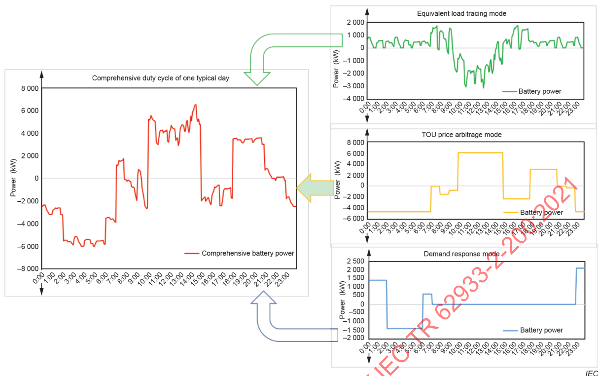
Figure 23 – EES duty cycle for the case of a business charging station based on common DC bus
