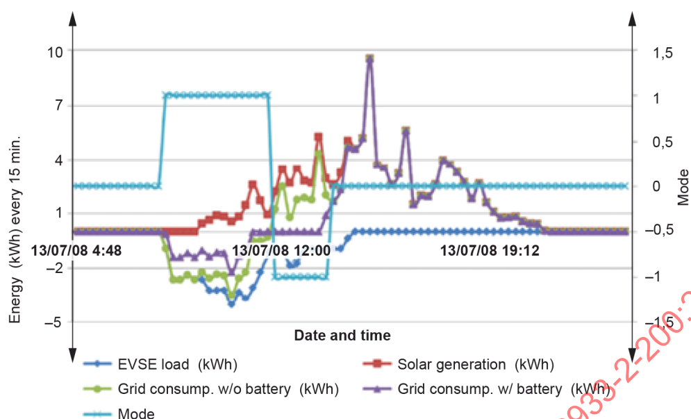
Figure 29 – Simulation results for operation strategy 3 for the case of a business charging station based on common AC bus
