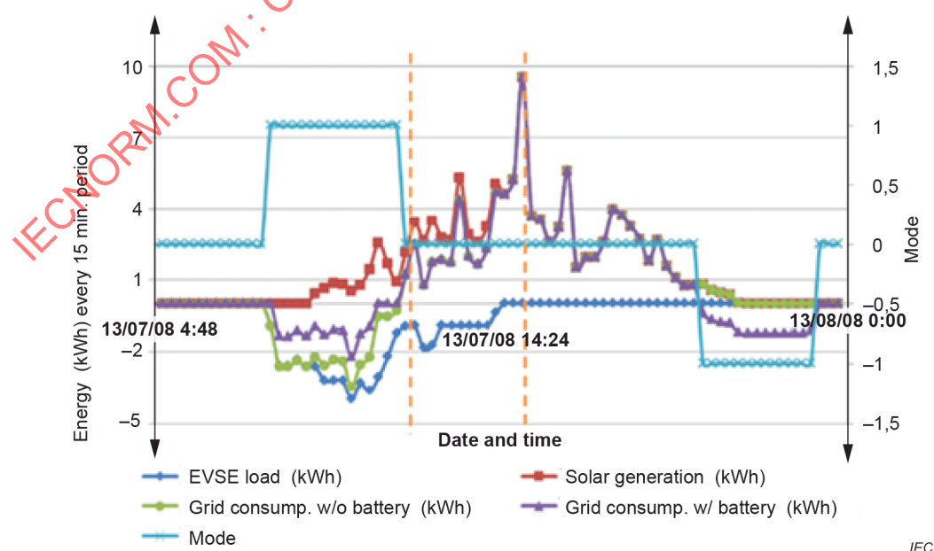
Figure 28 – Simulation results for operation strategy 2 for the case of a business charging station based on common AC bus
