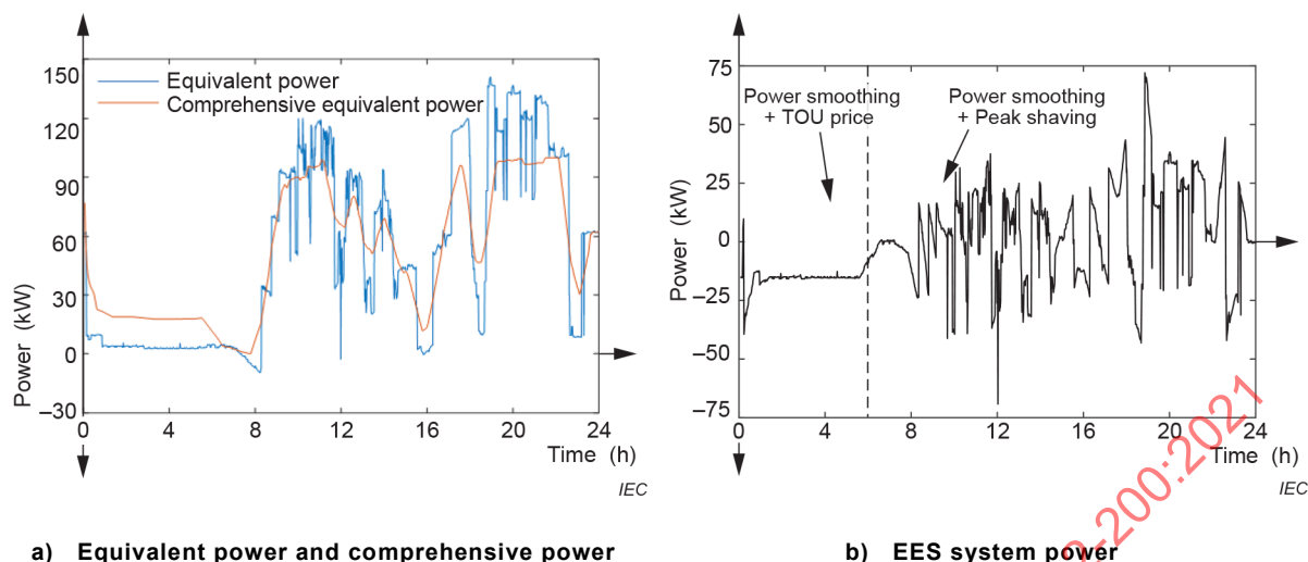
Figure 14 – EES duty cycle for the case of a commercial charging station based on common AC bus
