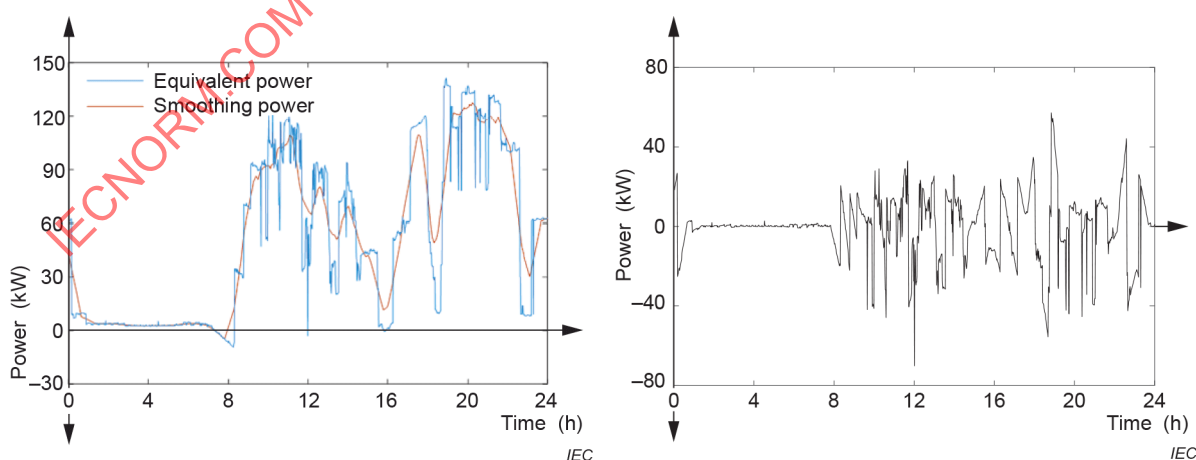
a) Equivalent power and smoothing power
