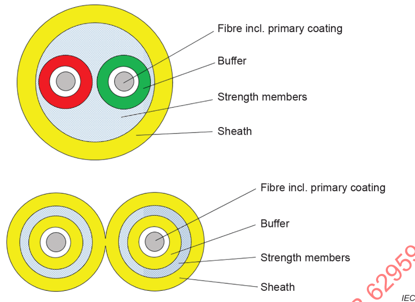
Figure D.6 – Duplex cable types
