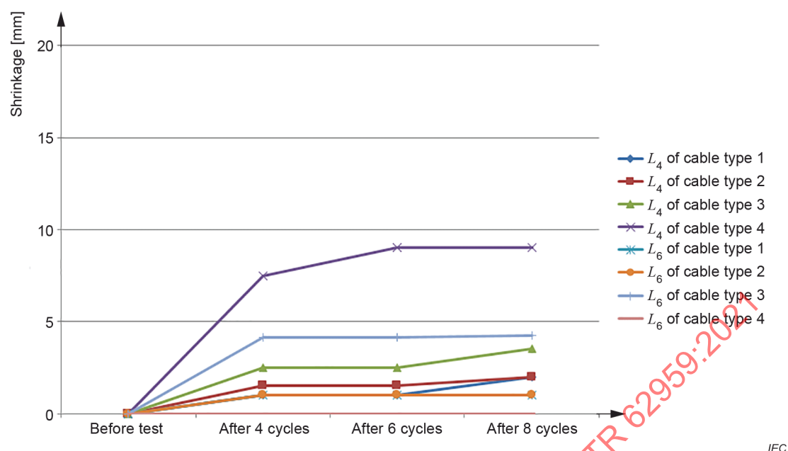
Figure A.8 – Shrinkage of sheath and loose tube after different number of cycles
