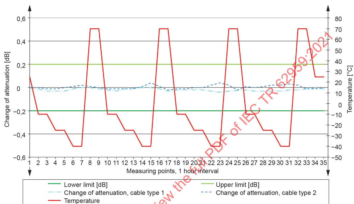
Figure A.5 – Change in attenuation during temperature cycling
