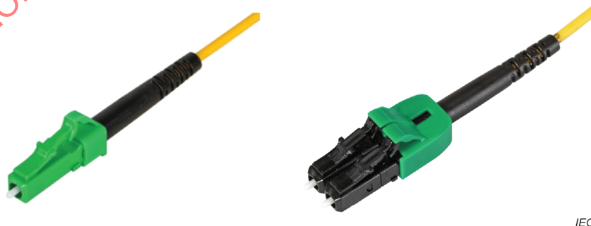
Figure D.2 – LC connector variants
