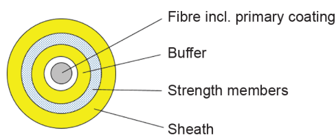
Figure D.5 – Simplex cable type
