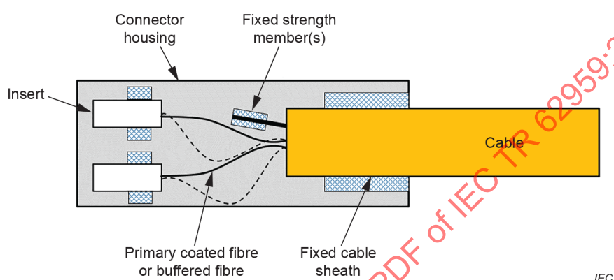
Figure E.1 – Cable terminated with hardened connector
