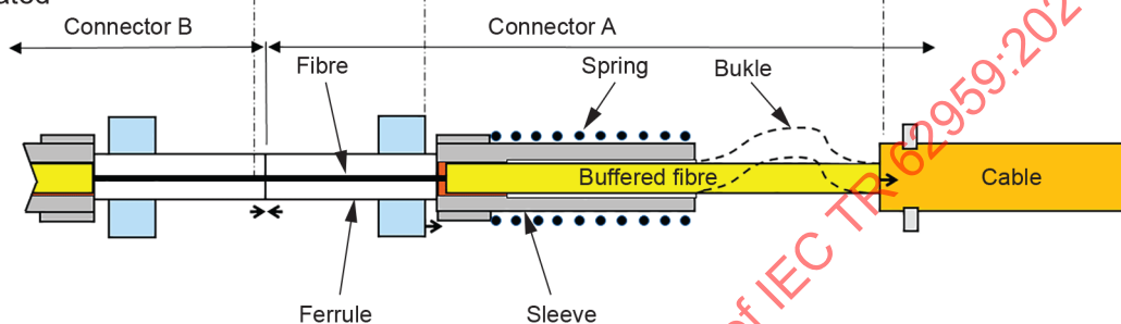
Figure D.4 – Fibre movement in spring-loaded connectors
