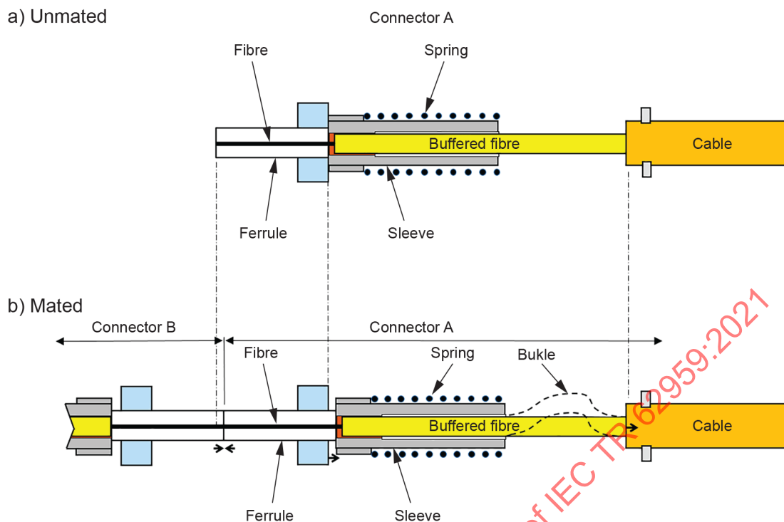
Figure D.4 – Fibre movement in spring-loaded connectors
