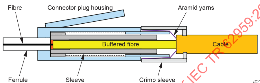
Figure D.1 – Cable terminated with connector plug
