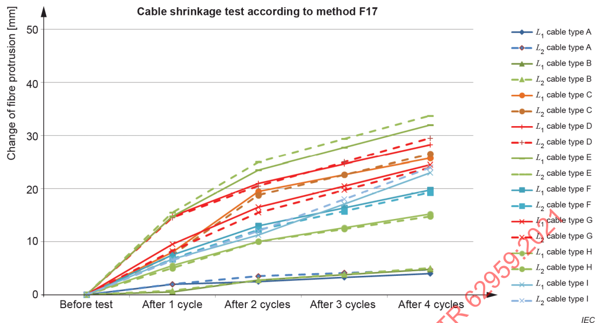
Figure A.14 – Change of fibre protrusion
