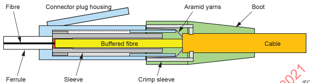
Figure D.3 – Simplex cable terminated at LC simplex connector
