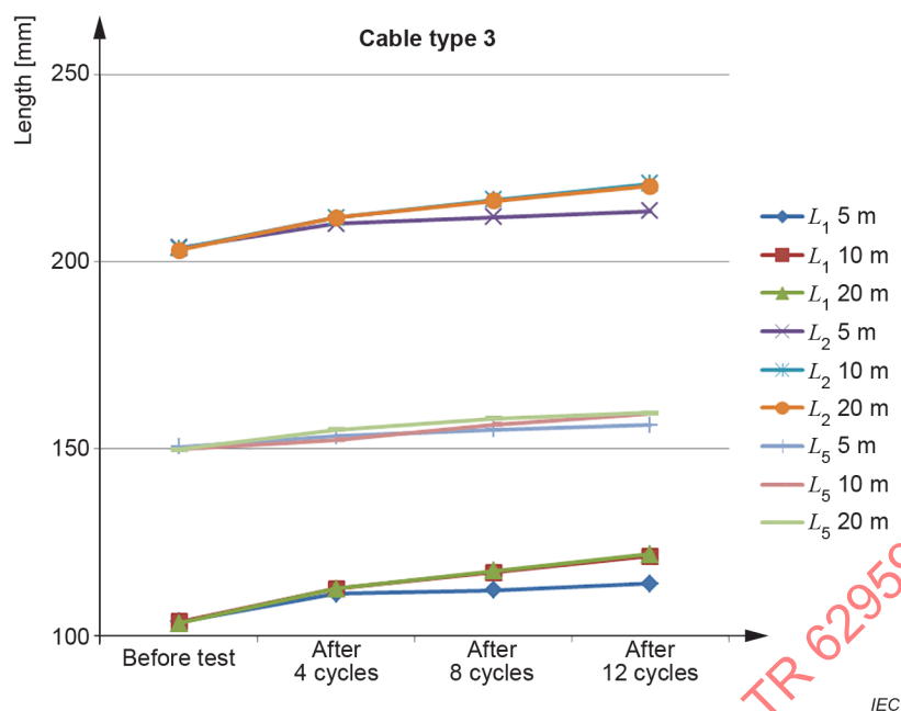
Figure A.12 – Protrusion length of cable type 3
