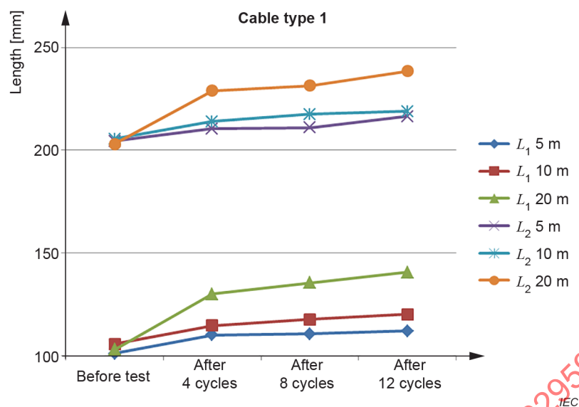
Figure A.10 – Protrusion length of cable type 1
