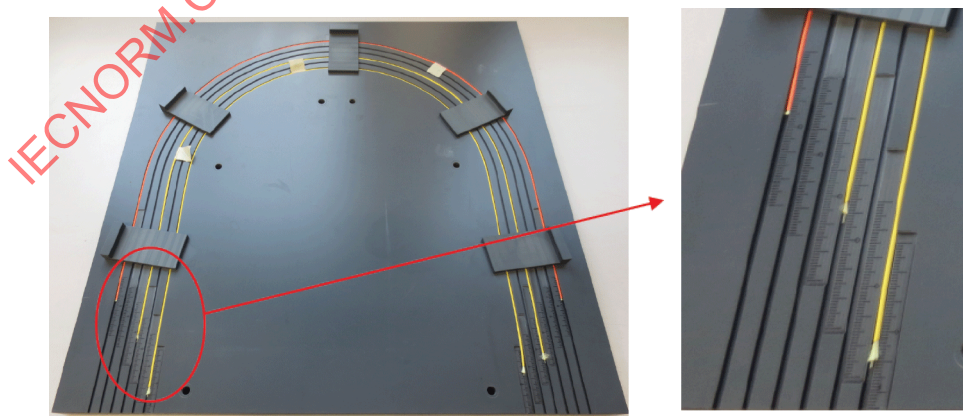
Figure B.1 – Apparatus for holding cable samples
