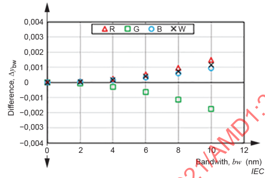
b) DUT-1 (chromaticity coordinate, y )
