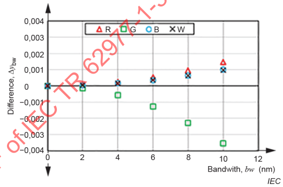
d) DUT-2 (chromaticity coordinate, y )
