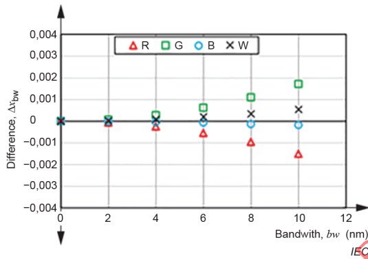
c) DUT-2 (chromaticity coordinate, x )
