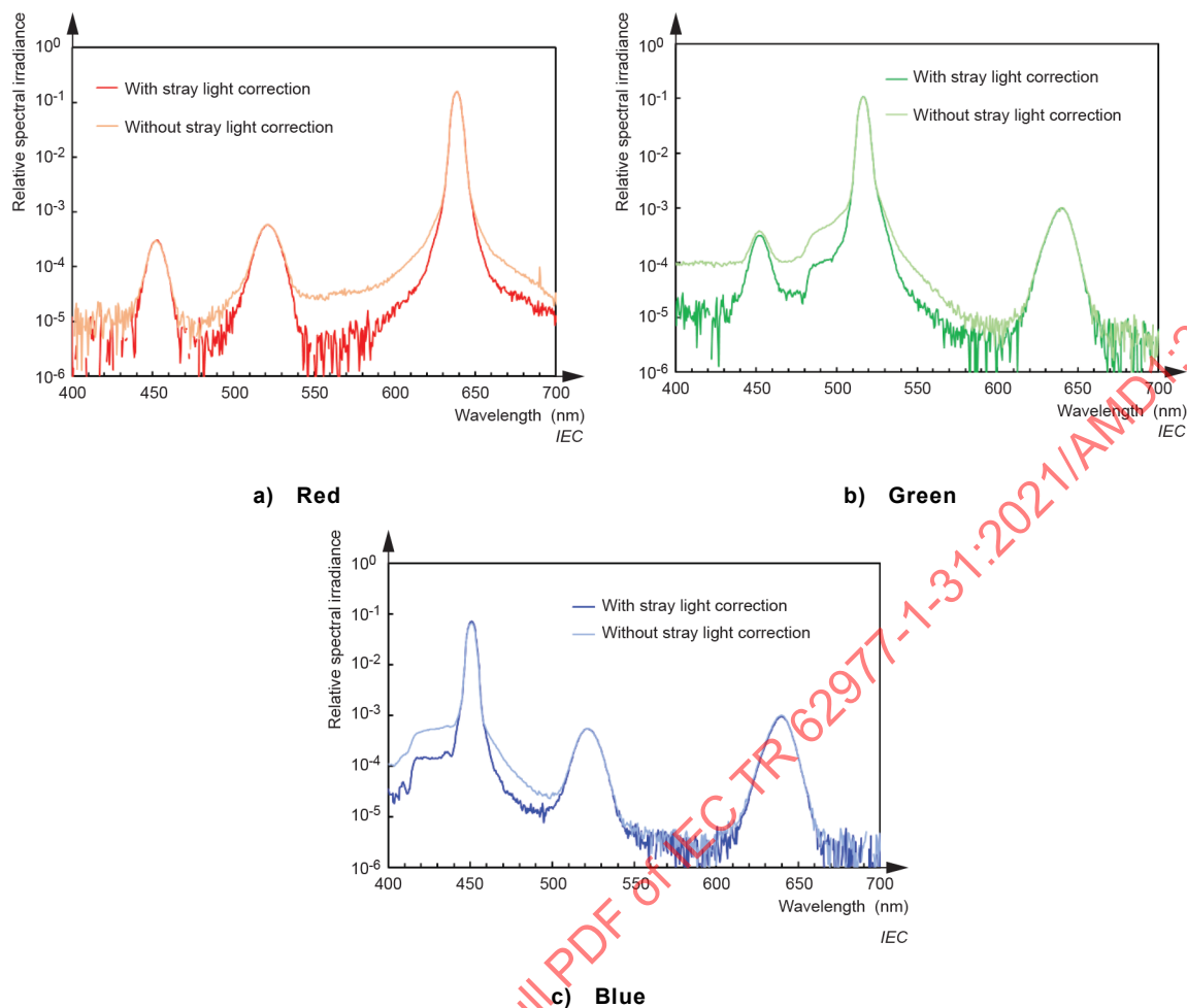
Figure E.1 – Measured relative spectral irradiance for each primary input signal
