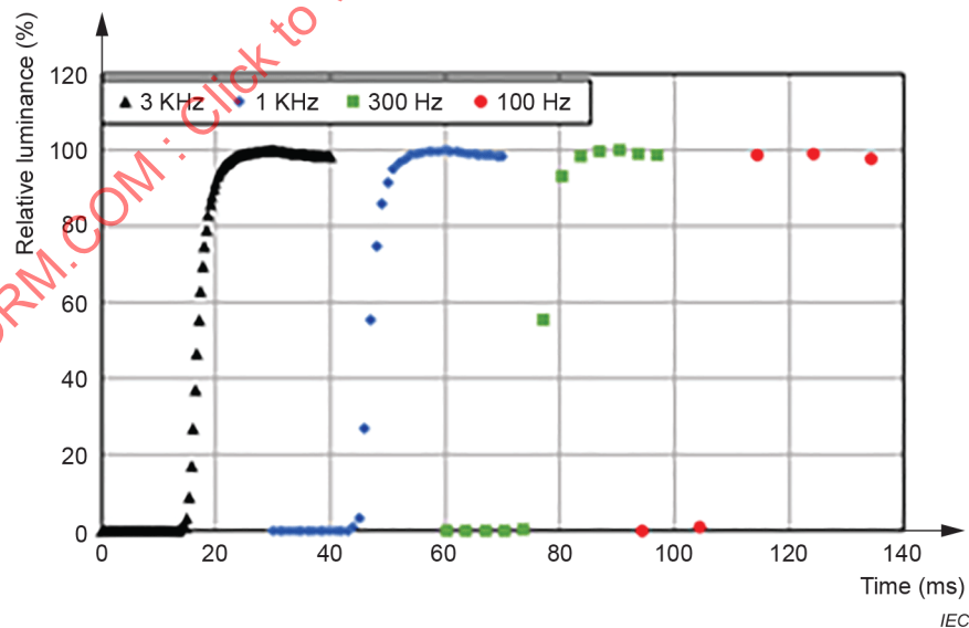
Figure 27 – Response curves measured at different sampling rates
