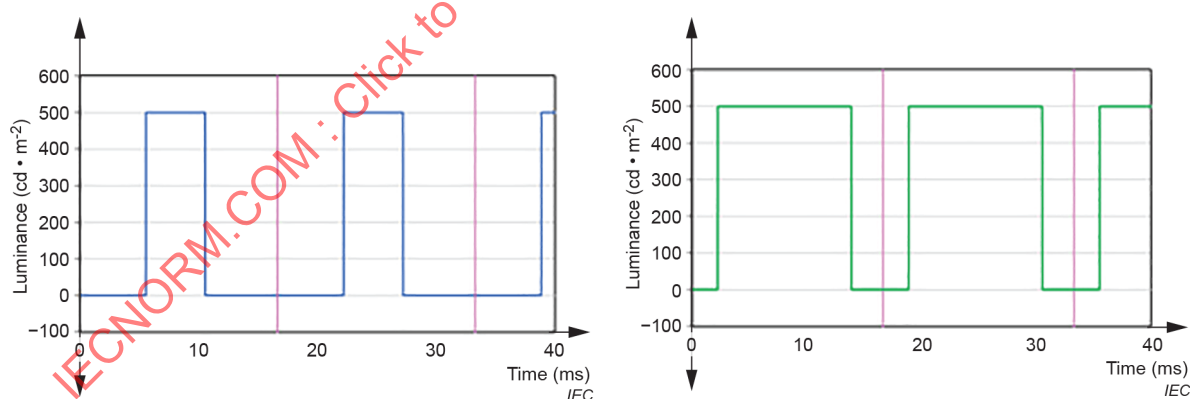
a) Frame duty cycle of 30 %
