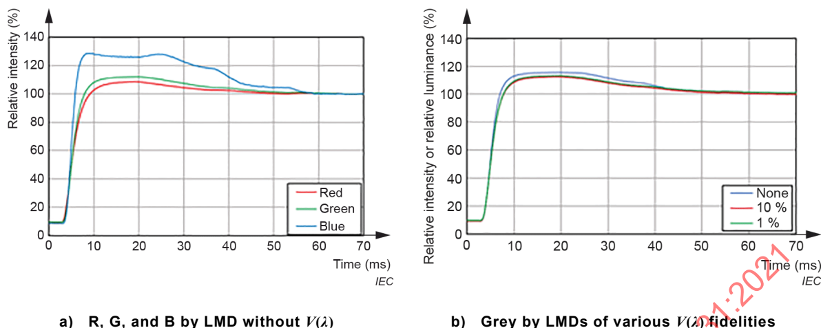
Figure 29 – Measured response curves switched from the 10 % to 90 % level
