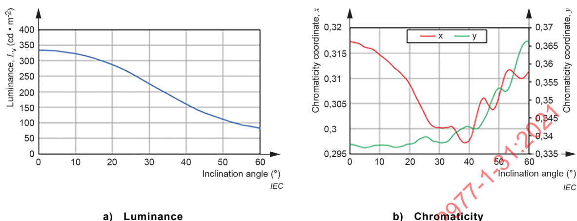
Figure C.2 – Inclination angle dependence
