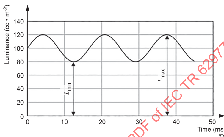
Figure 30 – Schematic measured temporal luminance modulation of the LCD with a common voltage offset
