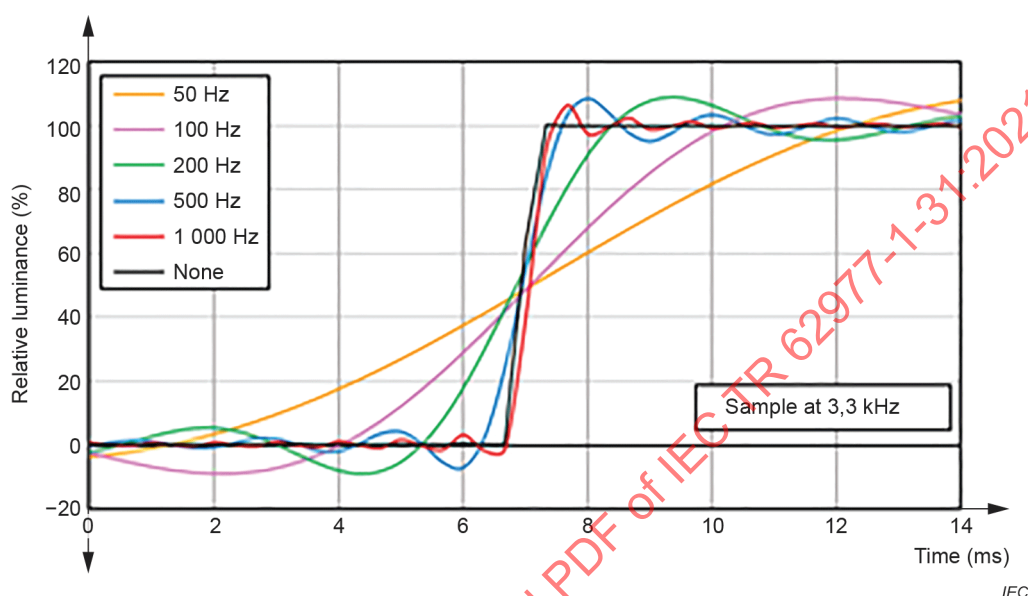
Figure 28 – Measured response subjected to various low-pass filterings
