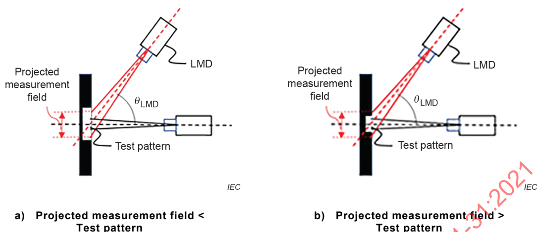
Figure 24 – Measurement field and test pattern
