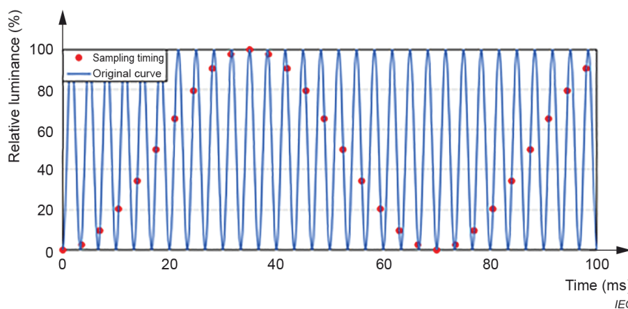
Figure 31 – Conceptual pseudo-temporal luminance modulation
