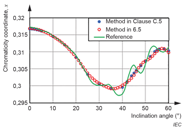
a) Chromaticity coordinate, x
