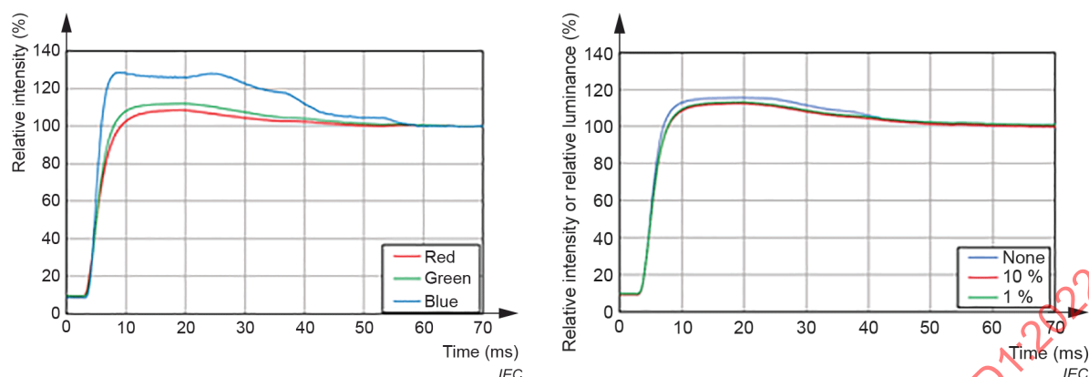
a) R, G, and B by LMD without V(\lambda)
