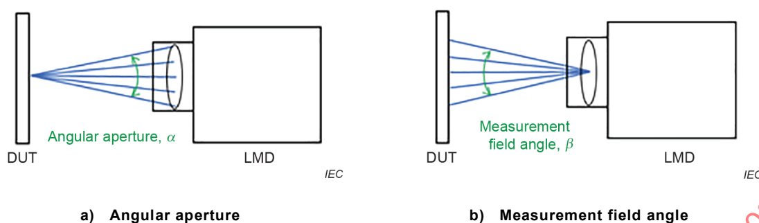
Figure 13 – Angular aperture and measurement field angle
