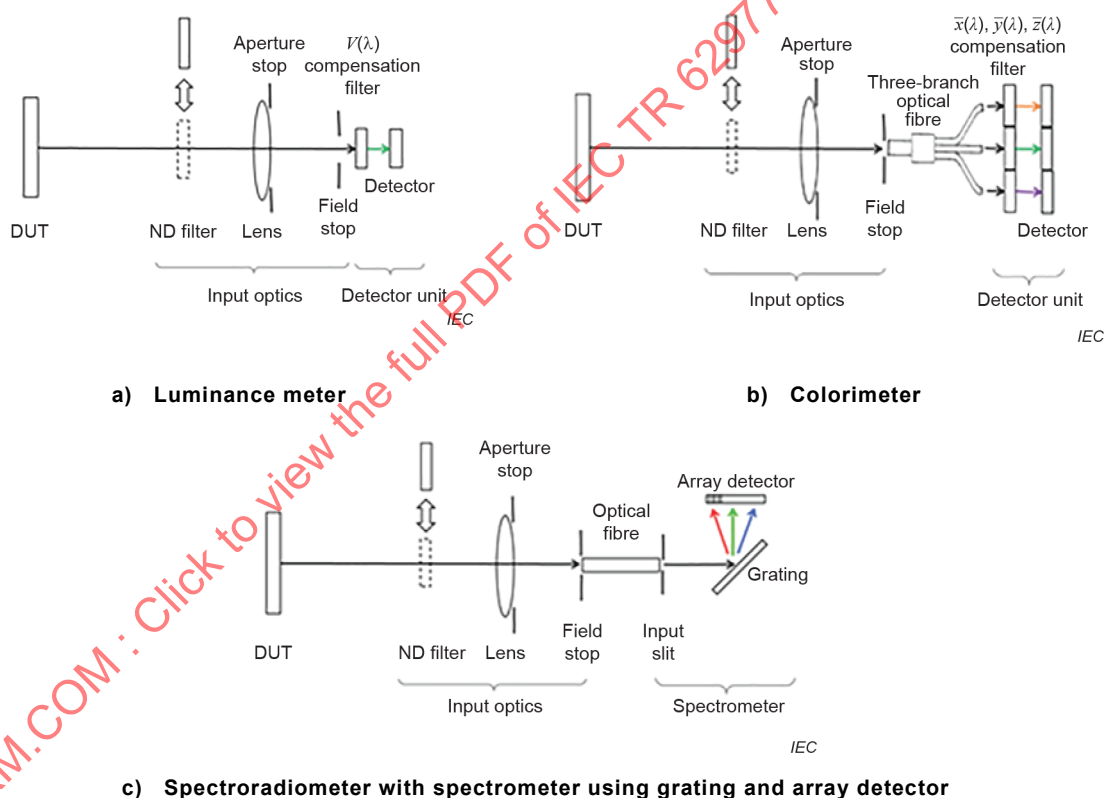
Figure 2 – Example of configurations for the input optics and detector
