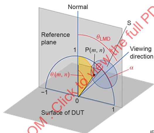
a) Inclination angle \theta(m, n) of the ray passing P(m, n) in circle S representing the angular aperture
