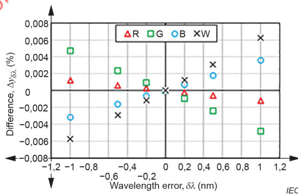
f) DUT-3 (chromaticity coordinate, y)
