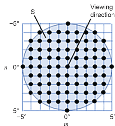
b) Points P(m, n) , shown as black dots, evenly distributed within the circle S
