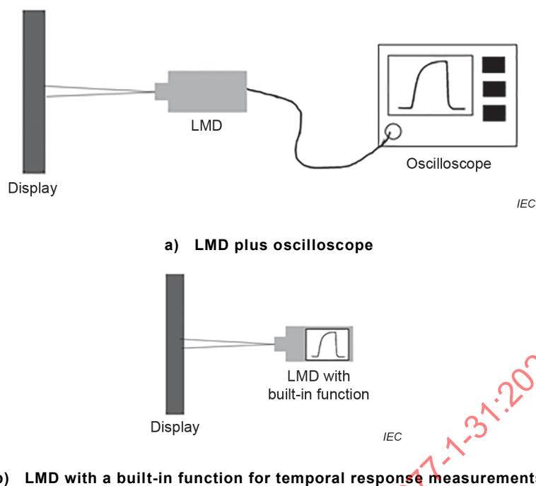
Figure 26 – Measurement setups for response time measurements
