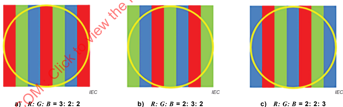
Figure C.7 – Three positions of a circular measurement field relative to the RGB stripes
