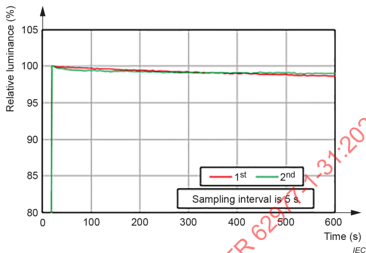
Figure D.2 – Changes of luminance after switching from the black to grey level
