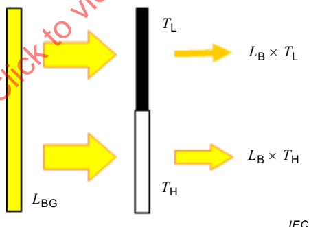
Figure 2 – On-screen contrast generated by electrically controlled transmittance, T_H and T_L
