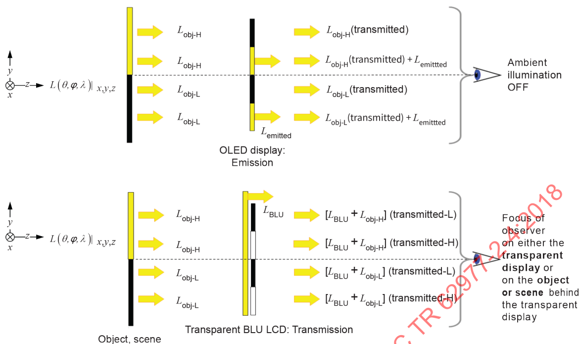
Figure 9 – Transparent display's scheme for OLED and LCD without background ambient illumination
