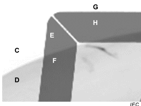
Figure 3 – Luminance image of a detail of Figure 1
