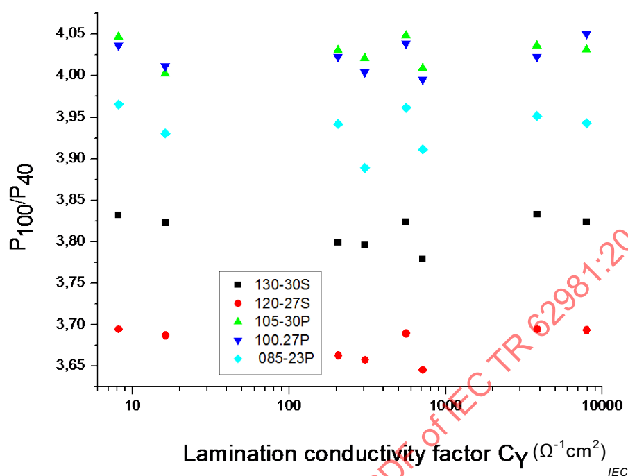
Figure 5 – Ratio of the power loss at 100 Hz to that at 40 Hz, P_{100}/P_{40} , at 1,7 T, versus lamination conductivity factor C_Y of the yokes
