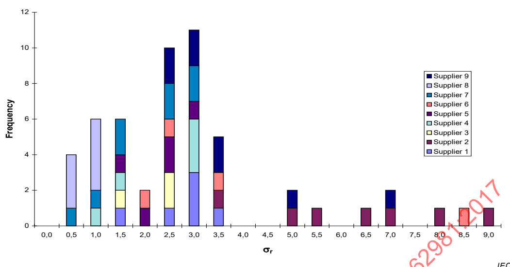
Figure 8 – Dispersion of manufacturer's grain-oriented material production in form of Epstein samples (PTB 1999)
