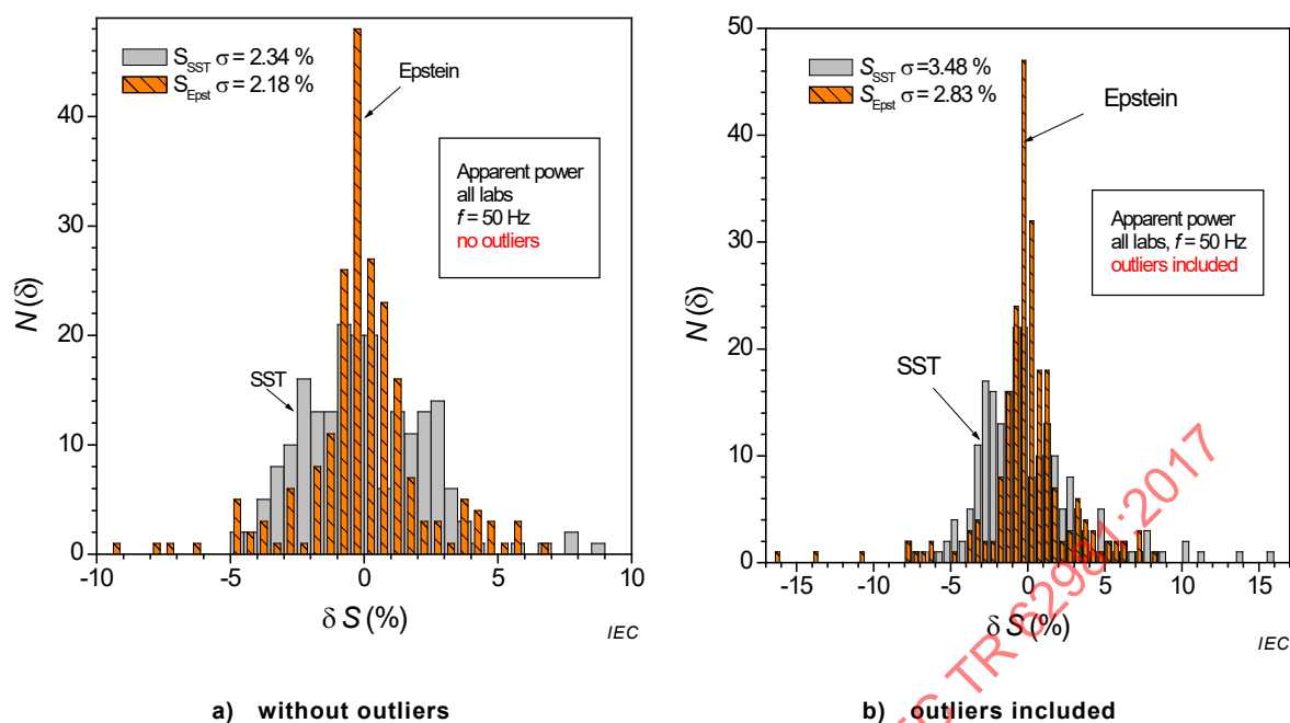
Figure 14 – Overall dispersion (all labs, J_p values, and samples) of the laboratories' best estimates S_i of the apparent power at 50 Hz around their reference values, with and without outliers
