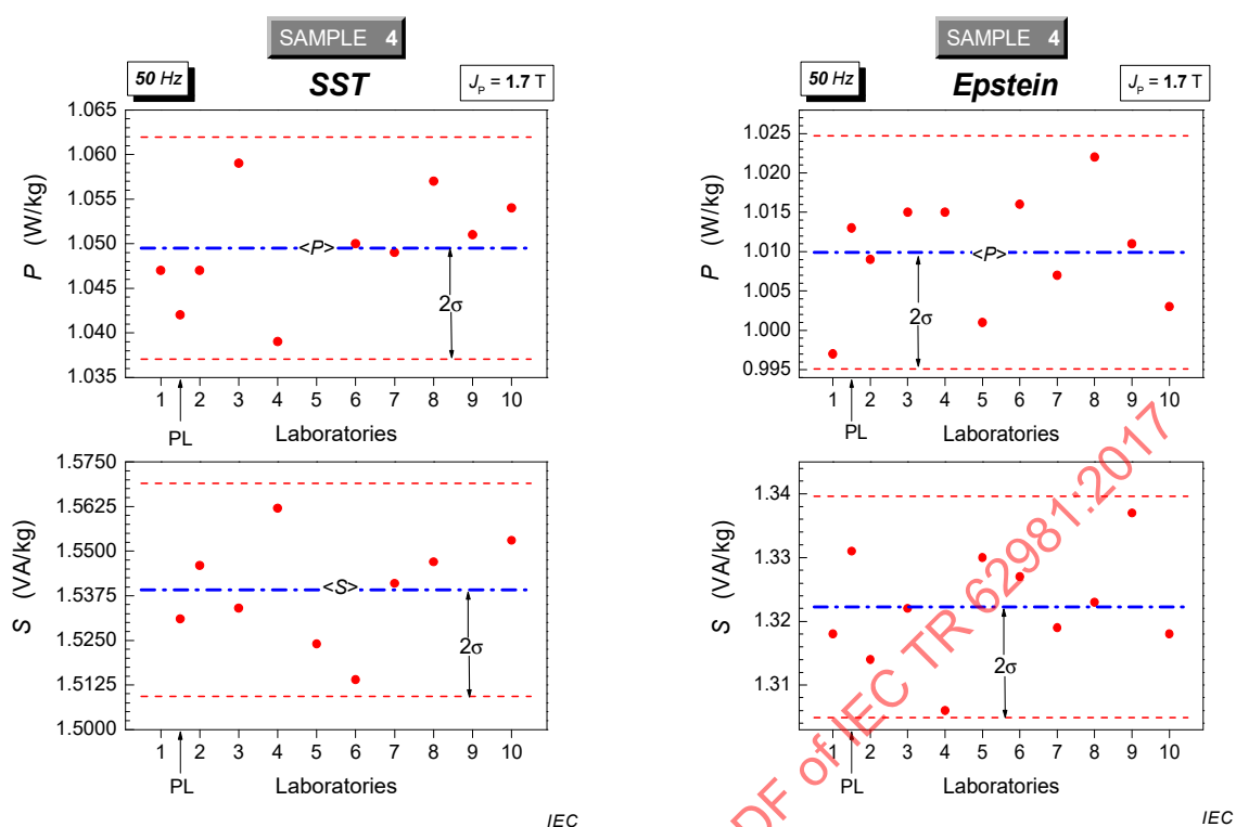
Figure 10 – Example of scattering of the laboratories' best estimates around the reference value (HGO sample No. 4, unweighted average, dash-dotted line)
