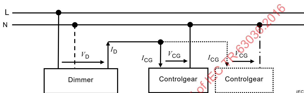
Figure 1 – Example of wiring diagram
