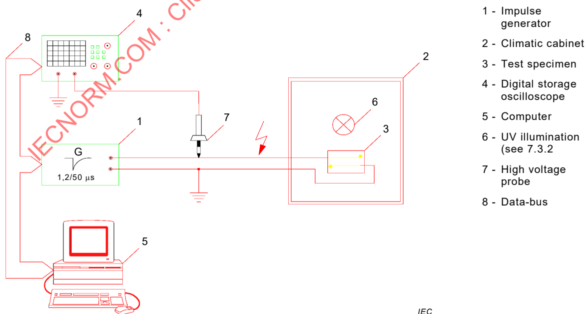
Figure 6 – Test circuit
