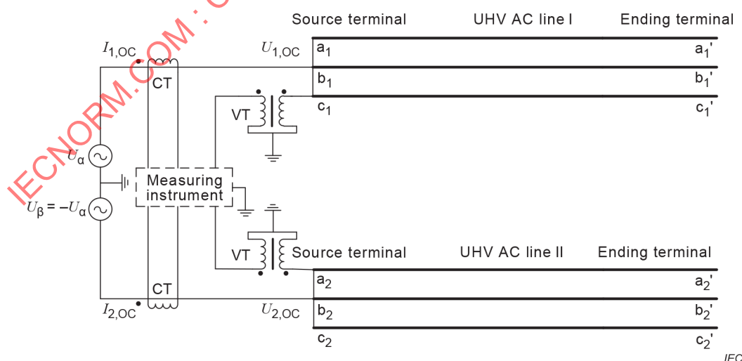
Figure 10 – Measurement of line-mode capacitance
