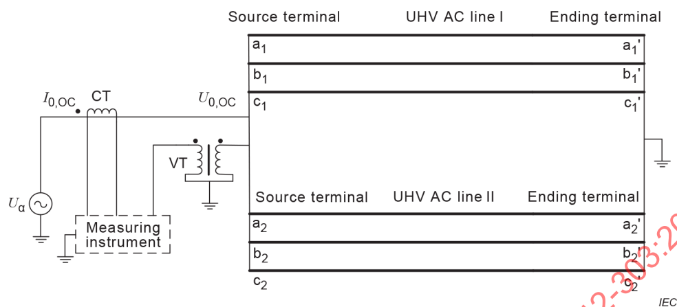
Figure 11 – Measurement of ground-mode impedance
