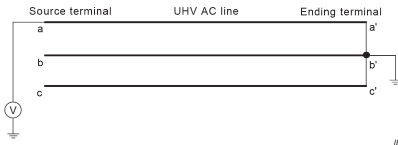
Figure 1 – Measurement of induced voltage
