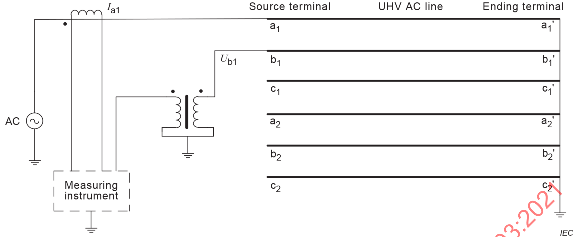
Figure 16 – Measurement of mutual impedance between two phases
