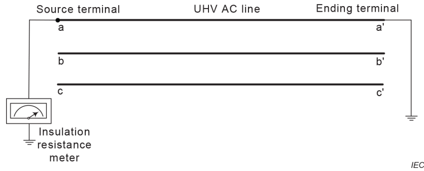
Figure 4 – Phase verification
