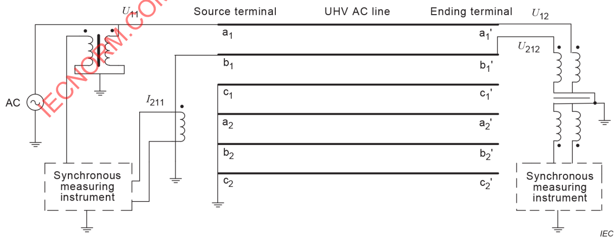
Figure 15 – Measurement of coupling capacitance between two phases
