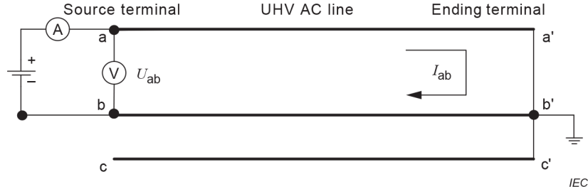
Figure 6 – Measurement of DC resistance
