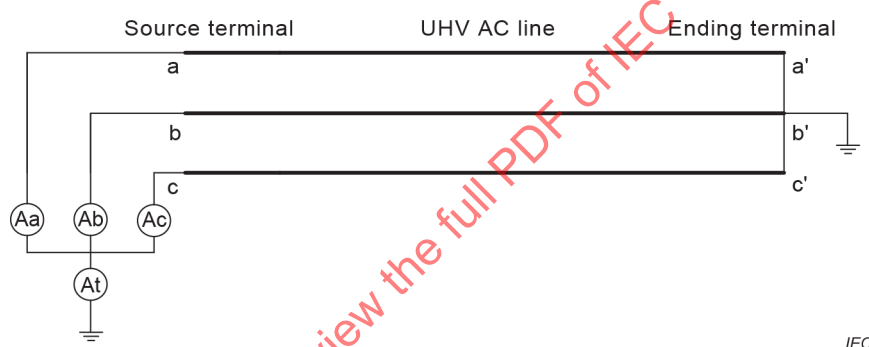
Figure 3 – Measurement of induced current
