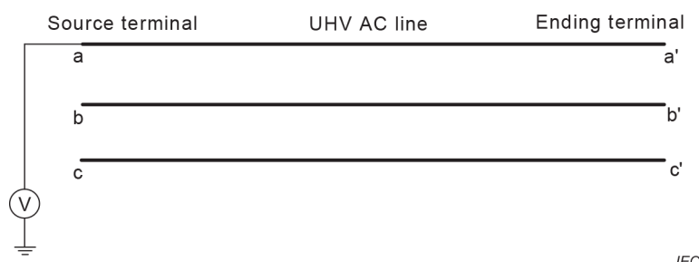
Figure 2 – Measurement of induced voltage
