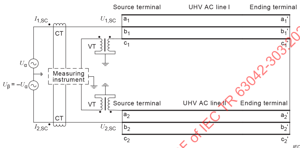
Figure 9 – Measurement of line-mode impedance
