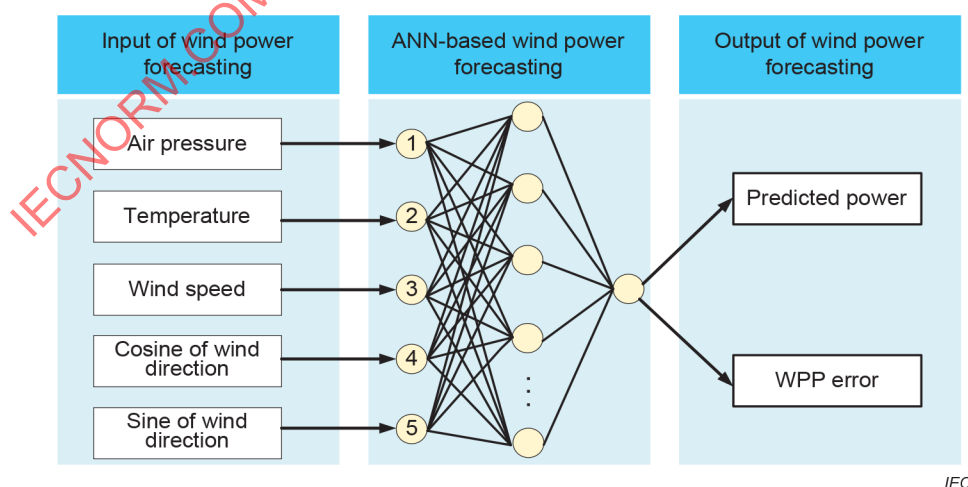
Figure 23 – Short-term WPF model based on ANN
