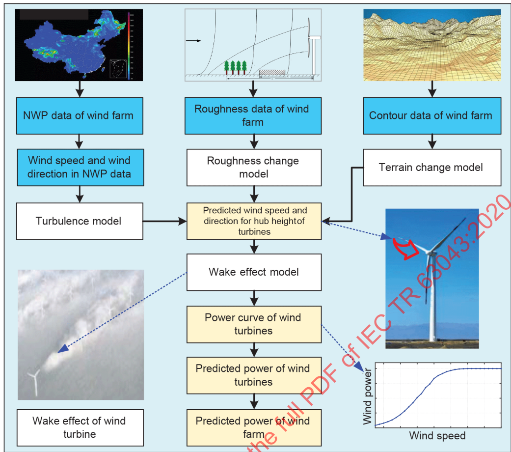
Figure 21 – Principle of short-term WPF based on physical approaches
