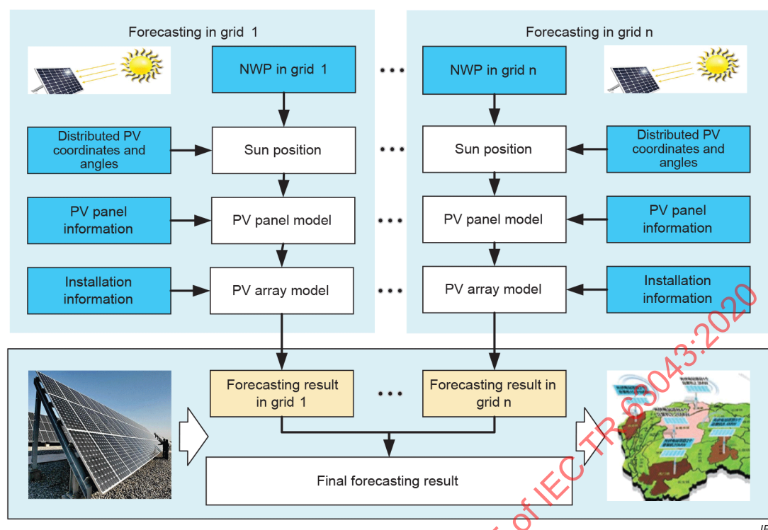
Figure 50 – Framework of grid forecasting method for distributed PVPF
