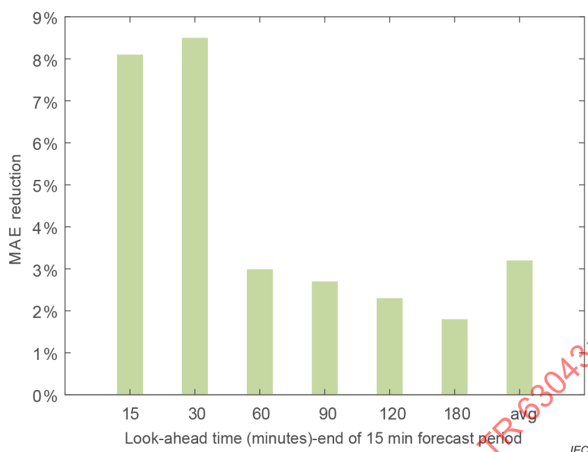
Figure 12 – Percentage MAE reduction by look-ahead time achieved by using the “rate of change” (indirect forecasting) versus “the 15 min average power generation” (direct forecasting) as the target predictand for the XGBoost model for 0 h to 3 h forecasts of the 15 min average TWRA aggregate (capacity of 2 319 MW) power production over the one year period from October 2015 to September 2016 [96]
