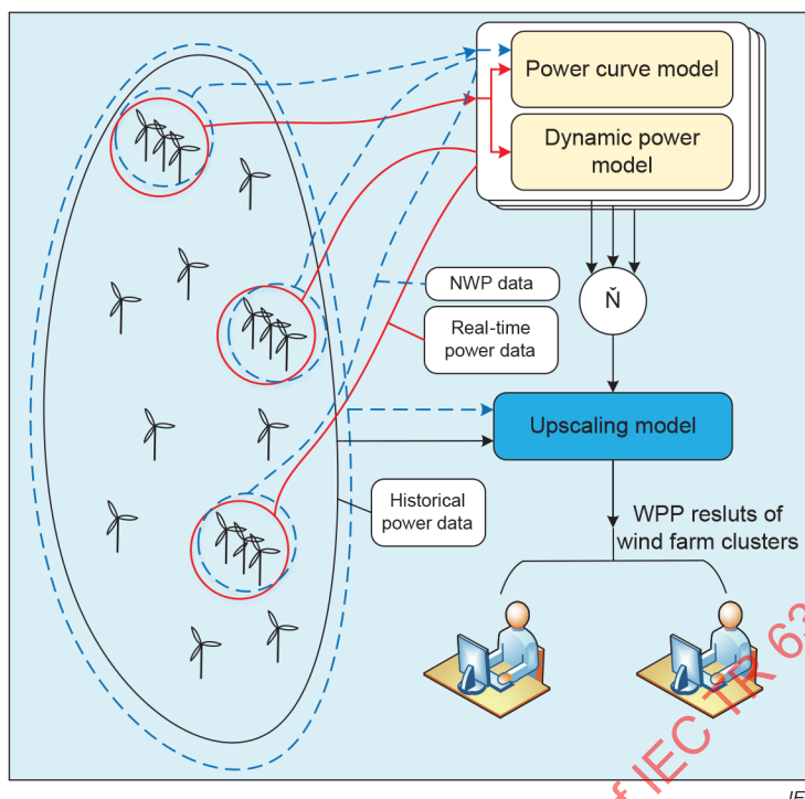
Figure 37 – Flow chart of the statistical upscaling method
