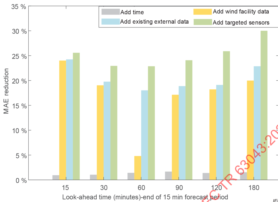
Figure 10 – Percentage MAE reduction over persistence by look-ahead time achieved by each source-dependent set of predictors for 0 h to 3 h forecasts of the 15 min average TWRA aggregate (capacity of 2 319 MW) power production over the one-year period from October 2015 to September 2016 [96]
