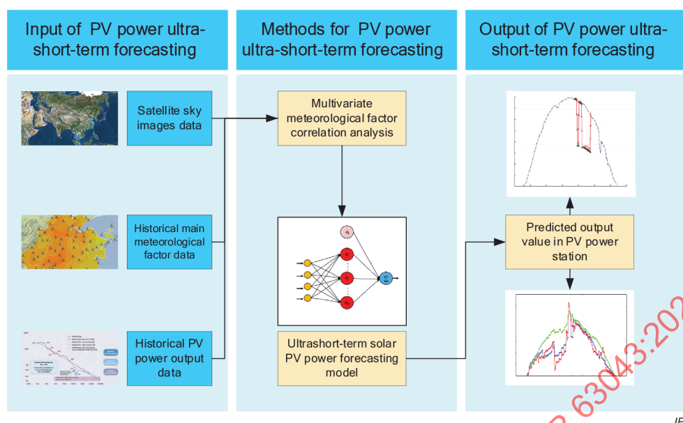
Figure 43 – Basic technology roadmap for pv power ultra-short-term forecasting
