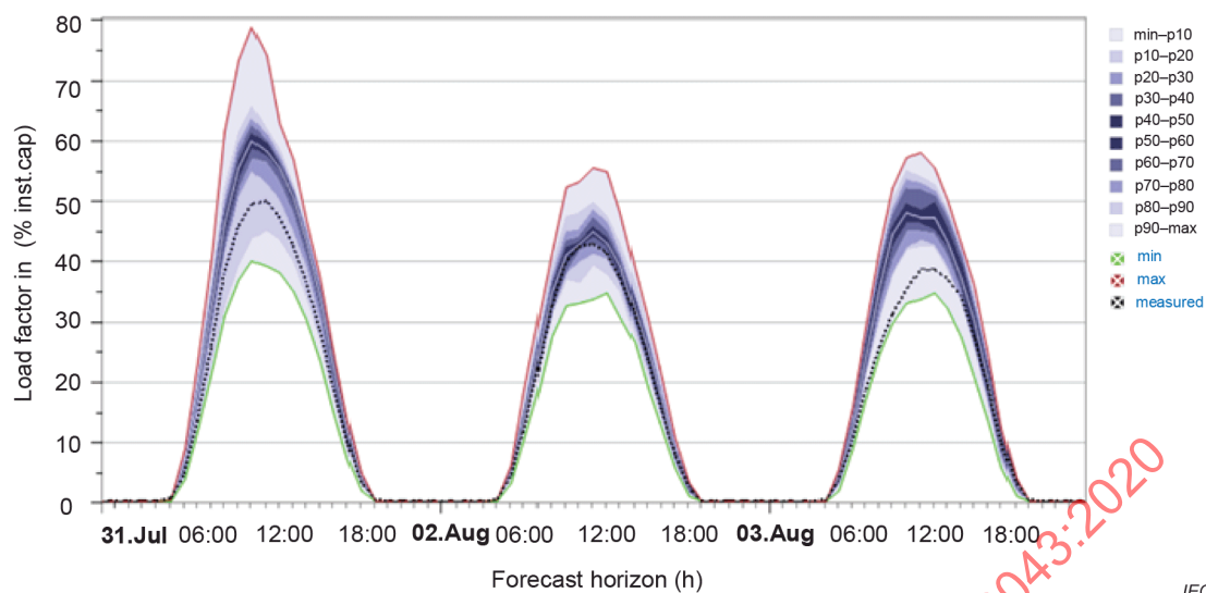
Figure 46 – Example of probabilistic PV model
