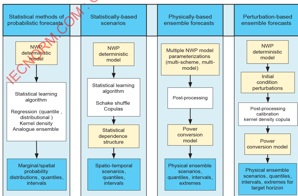
Figure 27 – Methods used for probabilistic forecasting
