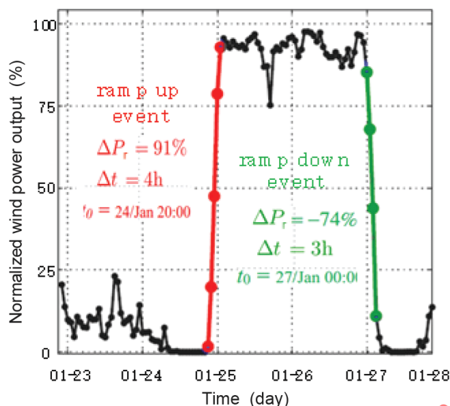
Figure 33 – Two ramp events of a wind farm
