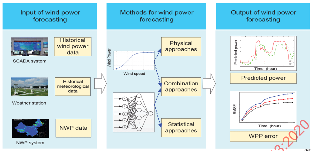
Figure 20 – Typical framework of short-term WPF
