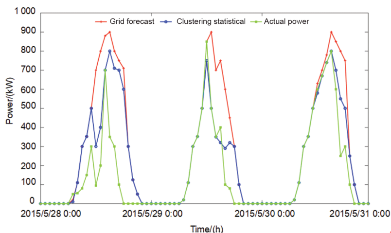
Figure 51 – Comparison between the forecasting results of the clustering statistical method and the grid forecast method
