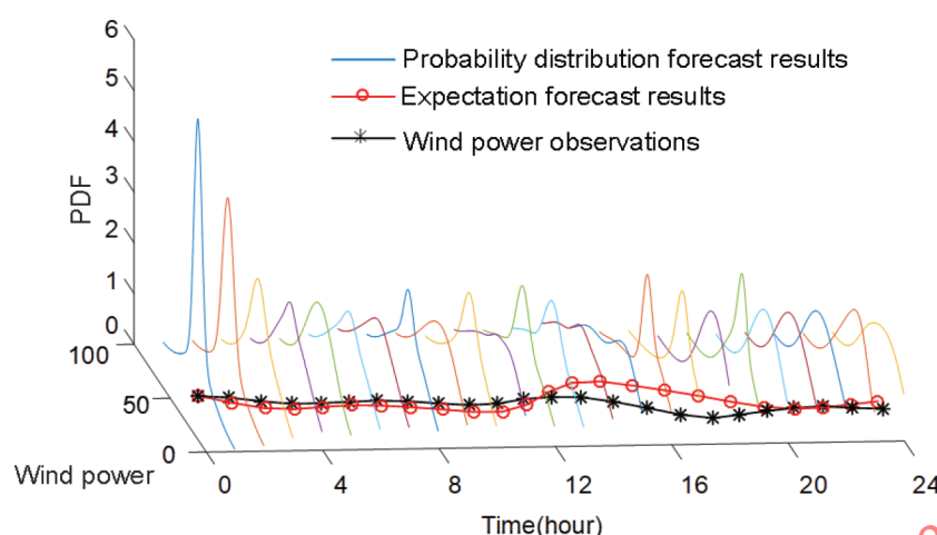
Figure 29 – Wind power probability distribution forecasting results
