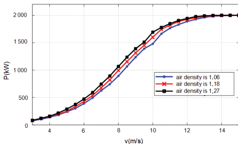
Figure 19 – Wind speed and wind power curves of wind turbines at different air densities
