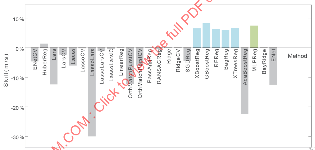
Figure 14 – Percentage reduction in the mean absolute error of NWP-based 0 h to 15 h wind power forecasts for the Tehachapi Wind Resource Area (TWRA) over a one-year period resulting from the application of 26 statistical forecasting methods to the output from the United States National Weather Service's High Resolution Rapid Refresh (HRRR) model [96]
