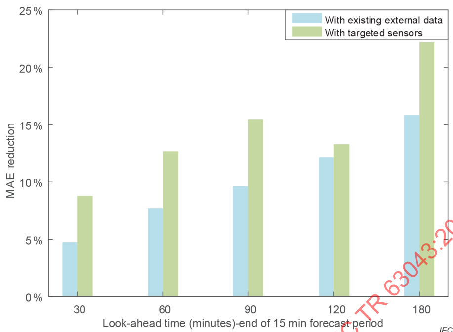
Figure 11 – Percentage MAE reduction by look-ahead time achieved by building forecasting models with the XGBoost method versus MLR for the “Add existing external data” (set #4) and “Add targeted sensors” (set #5) predictor sets for 0 h to 3 h forecasts of the 15 min average TWRA aggregate (capacity of 2 319 MW) power production over the one year period from October 2015 to September 2016 [96]
