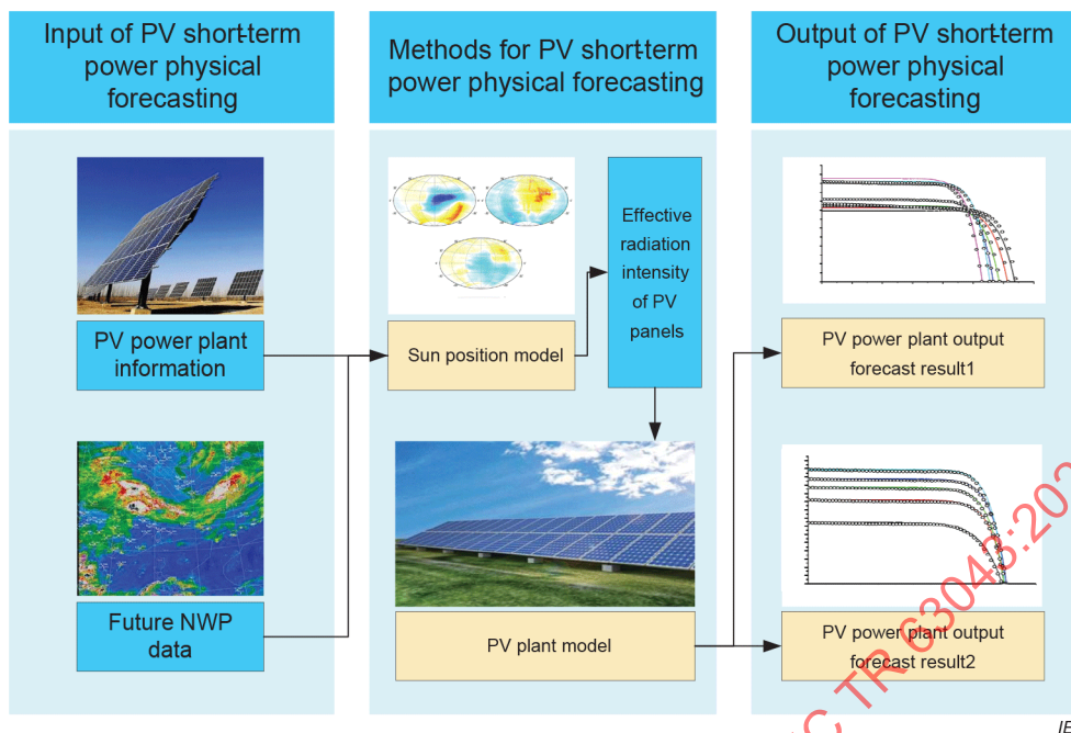
Figure 42 – PV short-term power physical forecasting method technical route
