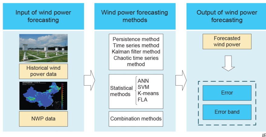
Figure 25 – Flowchart of ultra-short-term WPF
