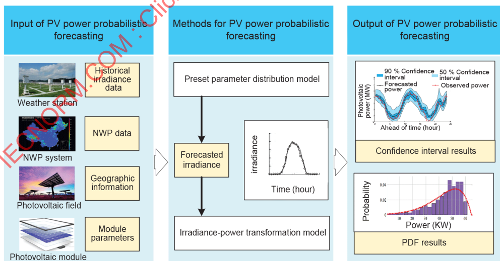
Figure 47 – Forecasting process of physical PV power probabilistic forecasting model
