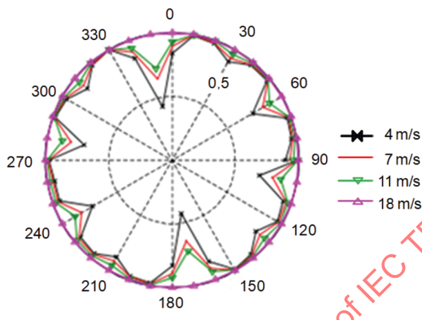
Figure 18 – EC distribution of a wind farm at different wind speeds and directions
