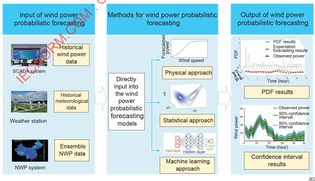
Figure 32 – Direct approach with ensemble NWP as input
