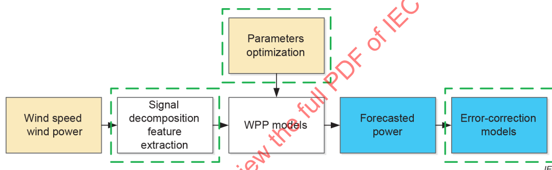
Figure 26 – Generalized combination methods of ultra-short-term WPF
