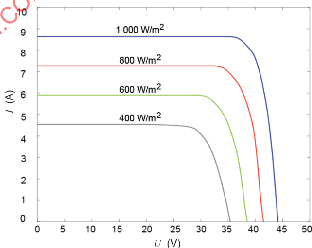
Figure 39 – Volt-ampere characteristic curve of PV modules corresponding to different irradiance
