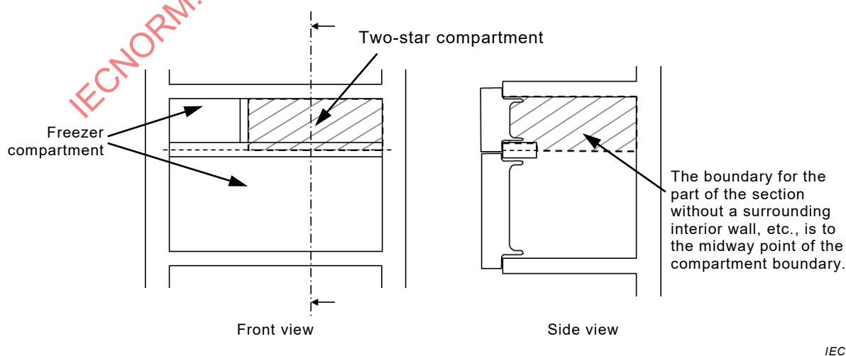
Figure B.2 – Part without partition in the freezer is a two-star compartment
