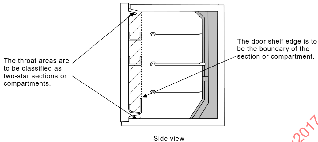
Figure B.3 – Freezer door shelves are a two-star section or compartment
