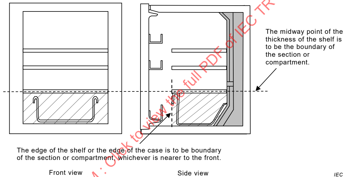
Figure B.4 – Drawer-type compartment in the freezer is a two-star section or compartment
