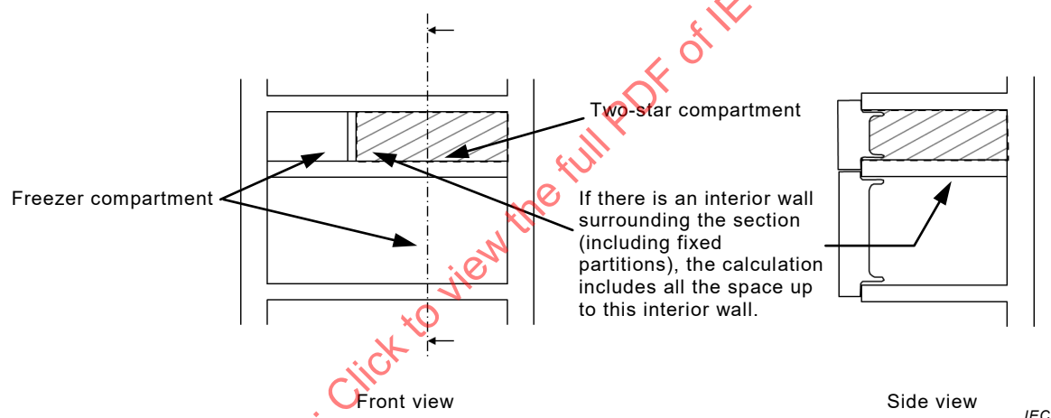
Figure B.1 – Part with partition in the freezer is a two-star compartment
