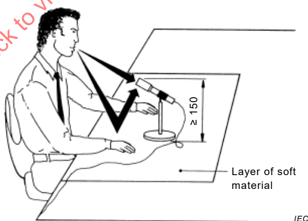
Figure 30 – Optimization of the height of the microphone above the table
