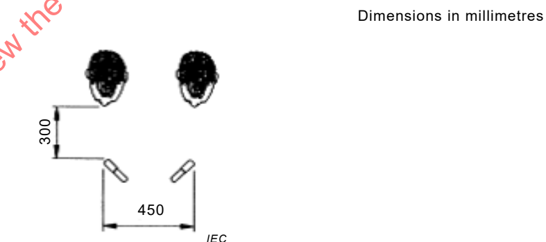
Figure 28 – A reduced 3-to-1 ratio using angled microphones
