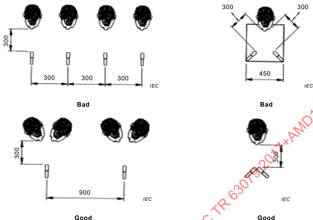
Figure 29 – Illustrations of good and bad microphone placements
