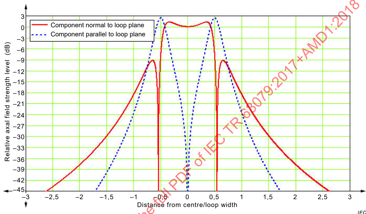
Figure F.1 – Magnetic field patterns
