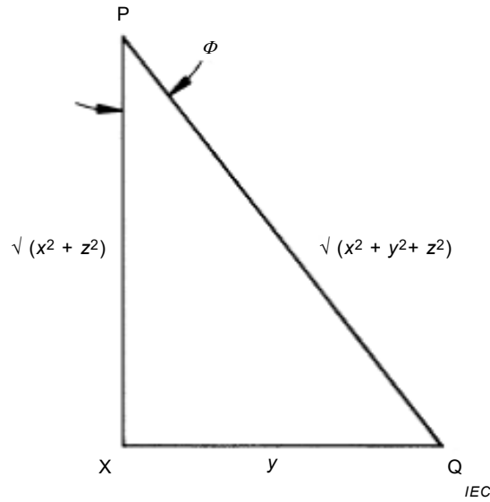
Figure C.4 – Diagram for calculating \cos \phi and \sin \phi
