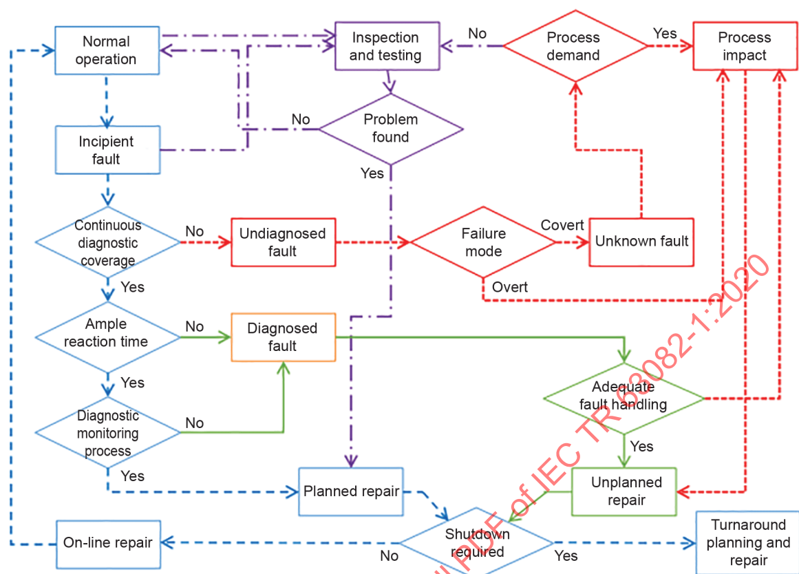
Figure 18 – State diagram for IDM diagnostics based maintenance processes
